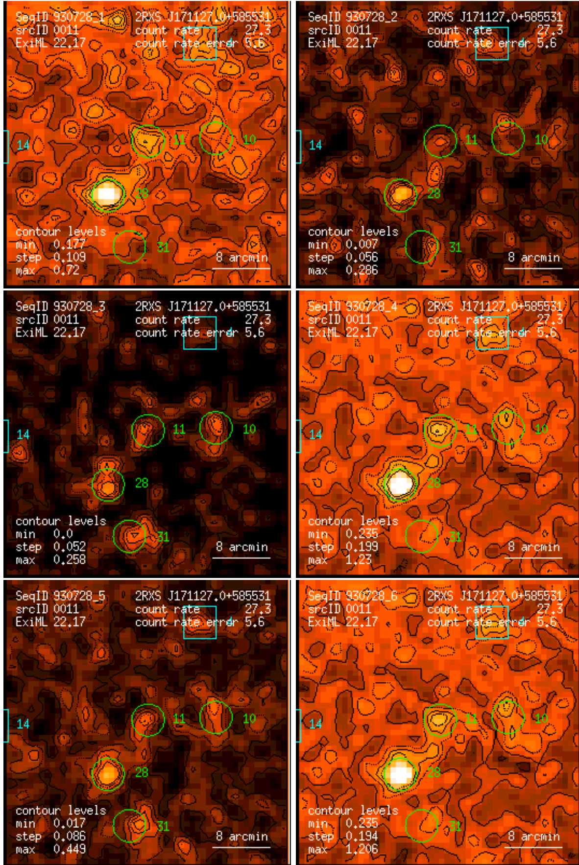
Figure 11: RASS 930728: detection 0011: band rate images, Gaussian filter: (1) PSPC channels 11 – 41, (2) 52 – 90, (3) 91 – 201, (4) 11 – 235, (5) 52 – 201, (6) 11 – 201. Broad band rates in counts/ks. Band rate contour levels in counts/ks/arcmin 2 .
