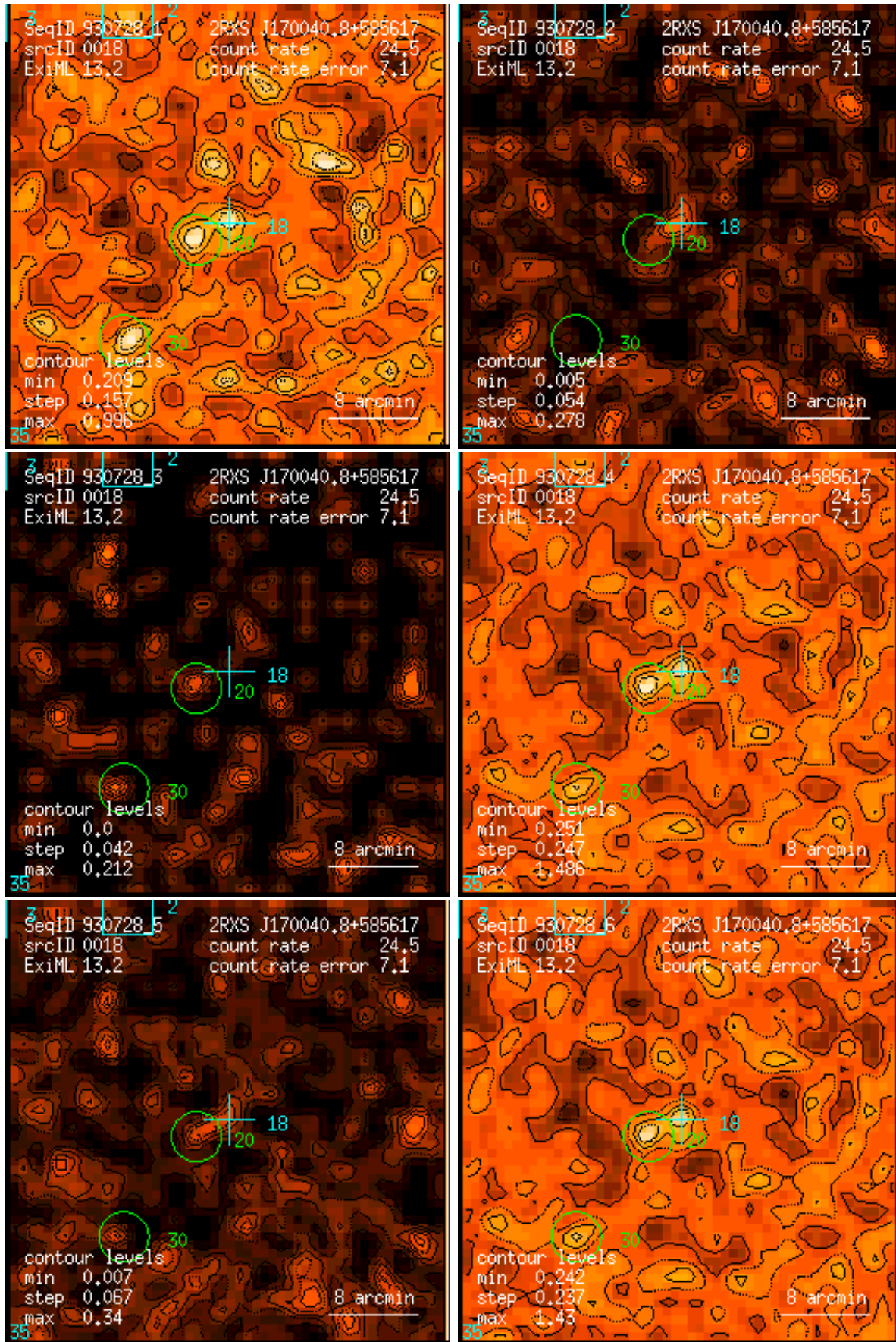
Figure 18: RASS 930728: detection 0018: band rate images, Gaussian filter: (1) PSPC channels 11 – 41, (2) 52 – 90, (3) 91 – 201, (4) 11 – 235, (5) 52 – 201, (6) 11 – 201. Broad band rates in counts/ks. Band rate contour levels in counts/ks/arcmin 2 .
