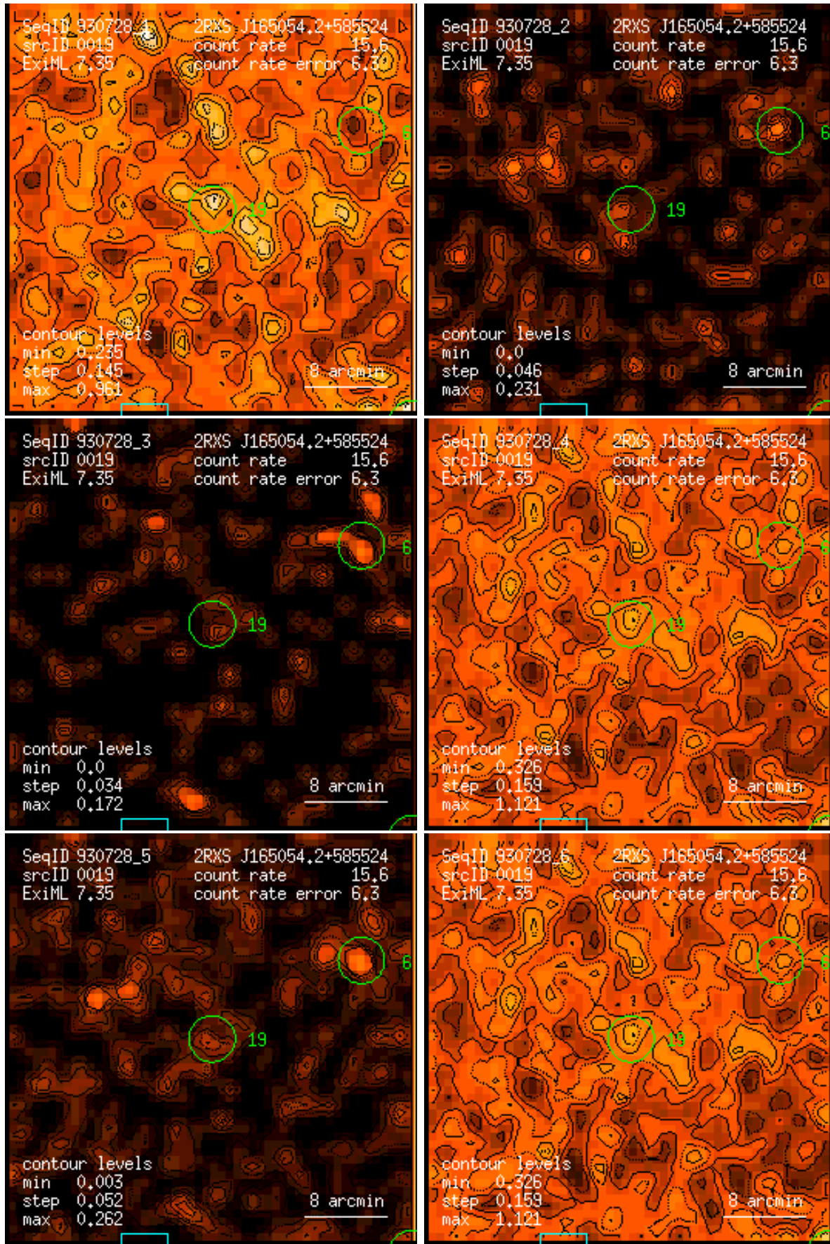
Figure 19: RASS 930728: detection 0019: band rate images, Gaussian filter: (1) PSPC channels 11 – 41, (2) 52 – 90, (3) 91 – 201, (4) 11 – 235, (5) 52 – 201, (6) 11 – 201. Broad band rates in counts/ks. Band rate contour levels in counts/ks/arcmin 2 .
