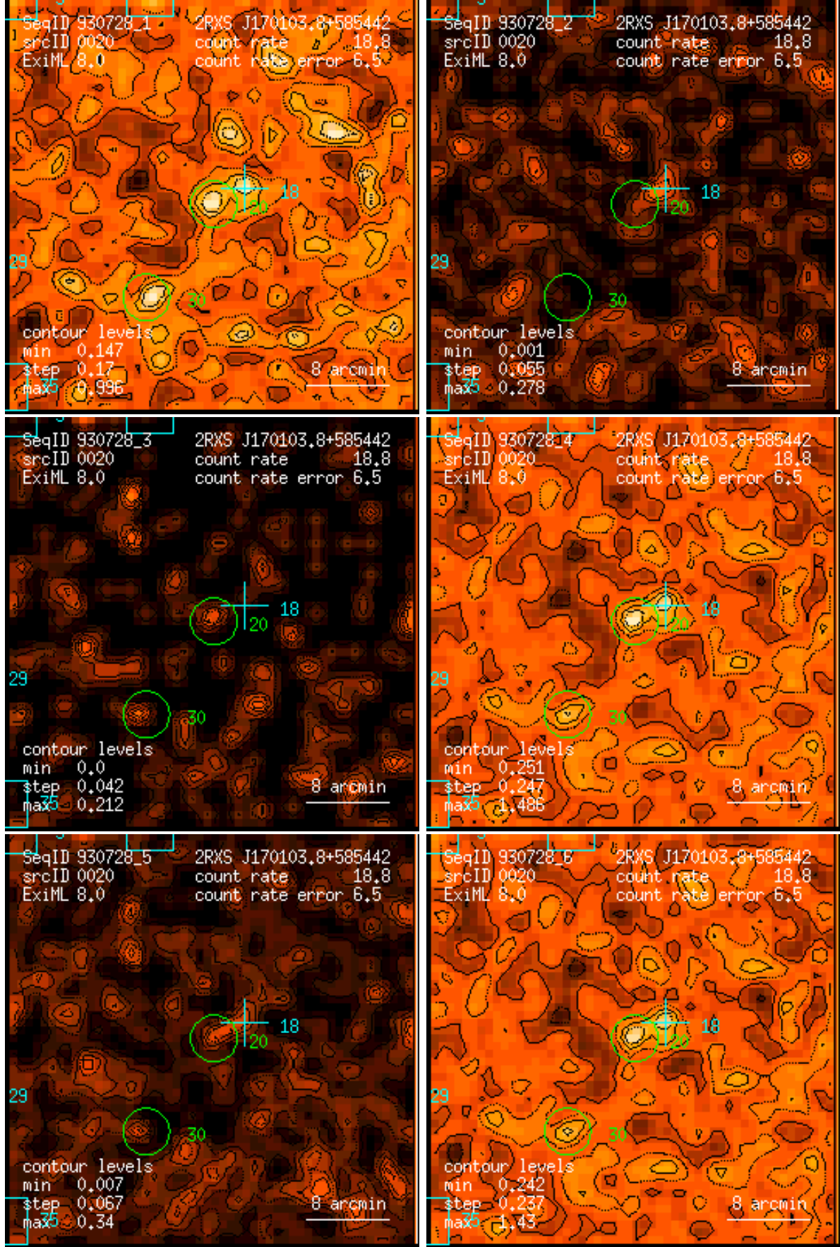
Figure 20: RASS 930728: detection 0020: band rate images, Gaussian filter: (1) PSPC channels 11 – 41, (2) 52 – 90, (3) 91 – 201, (4) 11 – 235, (5) 52 – 201, (6) 11 – 201. Broad band rates in counts/ks. Band rate contour levels in counts/ks/arcmin 2 .
