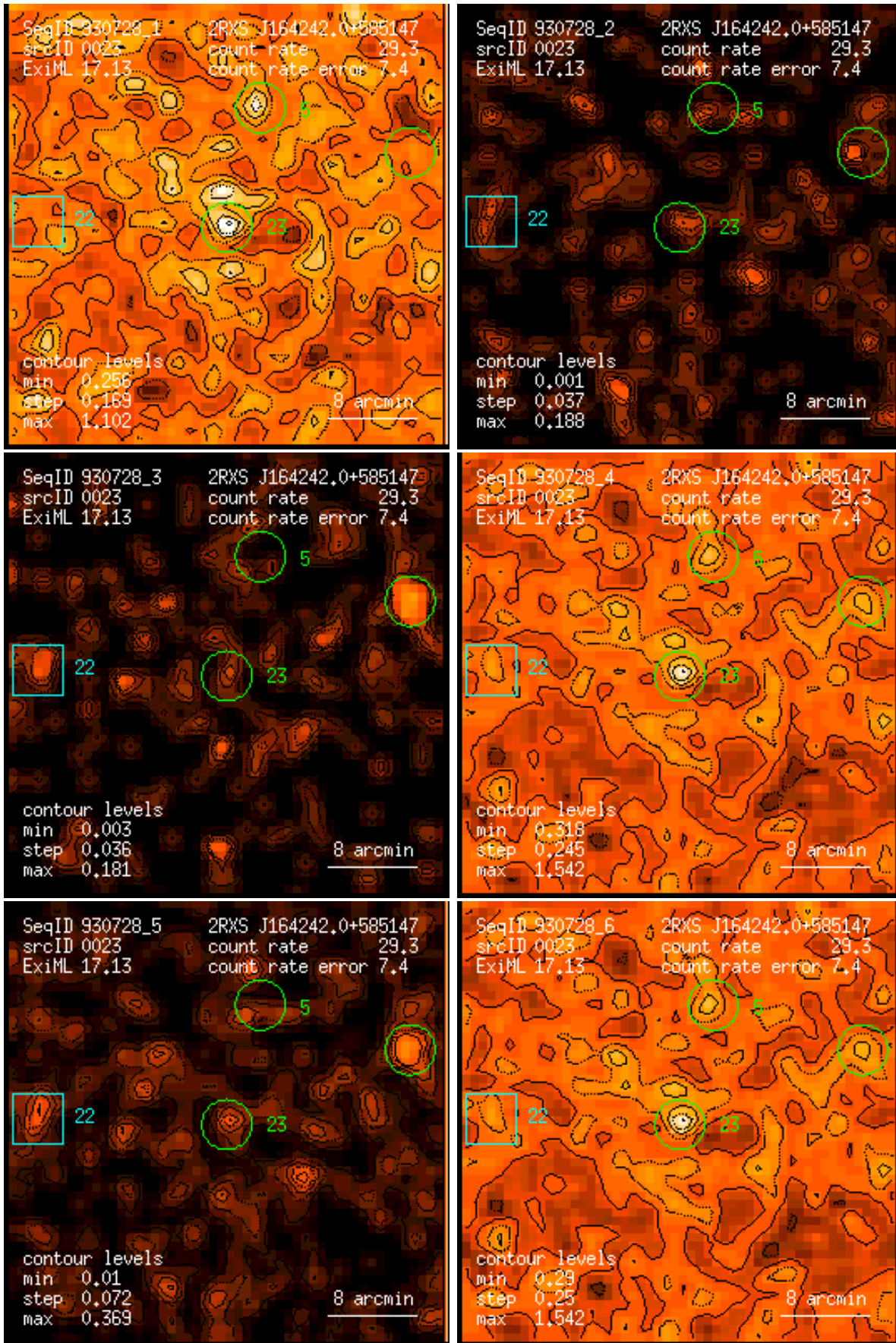
Figure 23: RASS 930728: detection 0023: band rate images, Gaussian filter: (1) PSPC channels 11 – 41, (2) 52 – 90, (3) 91 – 201, (4) 11 – 235, (5) 52 – 201, (6) 11 – 201. Broad band rates in counts/ks. Band rate contour levels in counts/ks/arcmin 2 .
