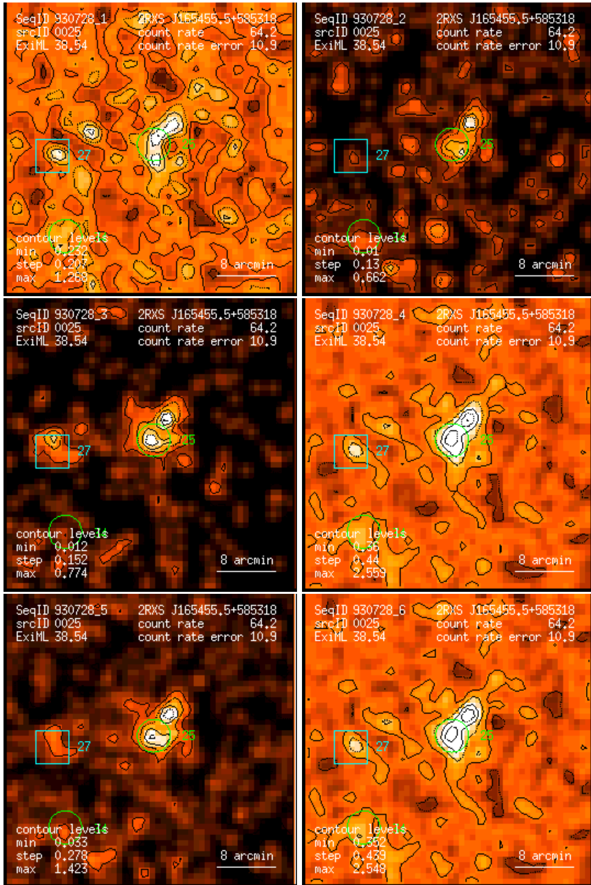
Figure 25: RASS 930728: detection 0025: band rate images, Gaussian filter: (1) PSPC channels 11 – 41, (2) 52 – 90, (3) 91 – 201, (4) 11 – 235, (5) 52 – 201, (6) 11 – 201. Broad band rates in counts/ks. Band rate contour levels in counts/ks/arcmin 2 .
