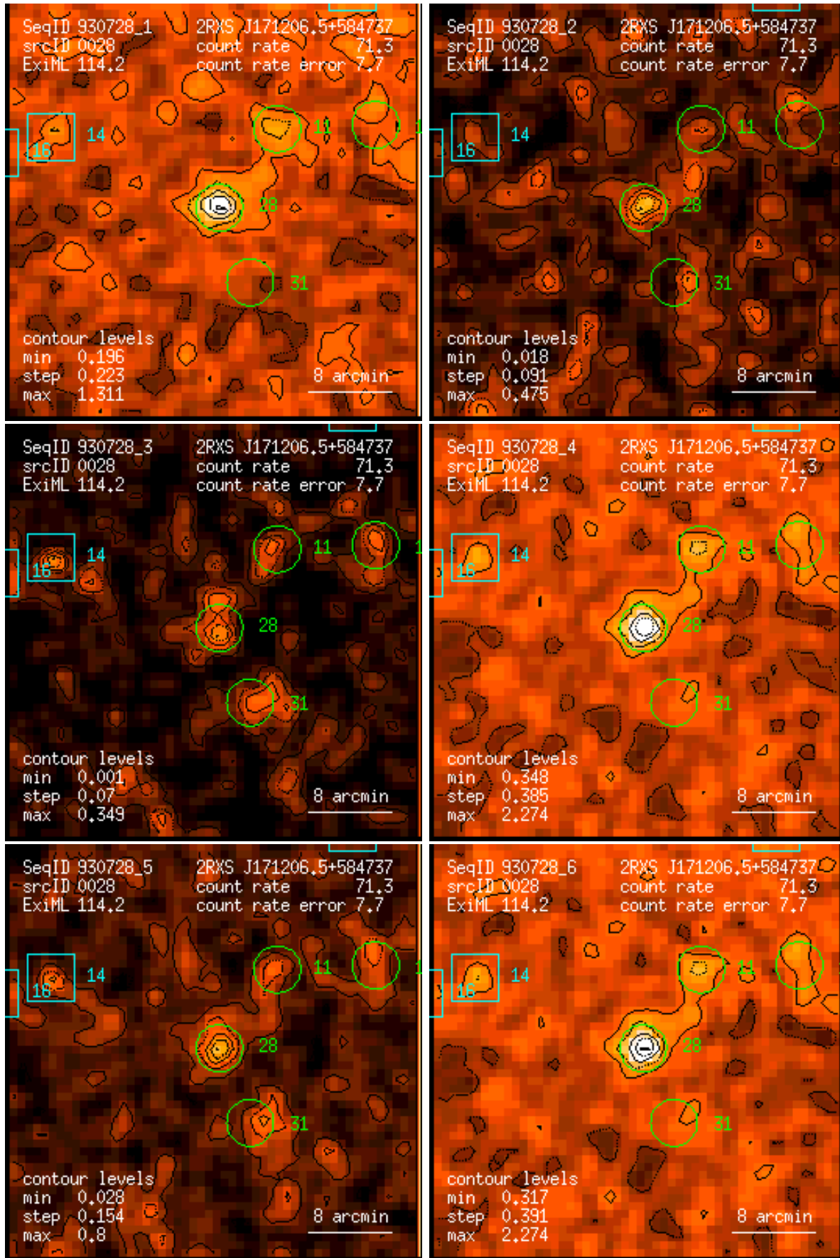
Figure 28: RASS 930728: detection 0028: band rate images, Gaussian filter: (1) PSPC channels 11 – 41, (2) 52 – 90, (3) 91 – 201, (4) 11 – 235, (5) 52 – 201, (6) 11 – 201. Broad band rates in counts/ks. Band rate contour levels in counts/ks/arcmin 2 .
