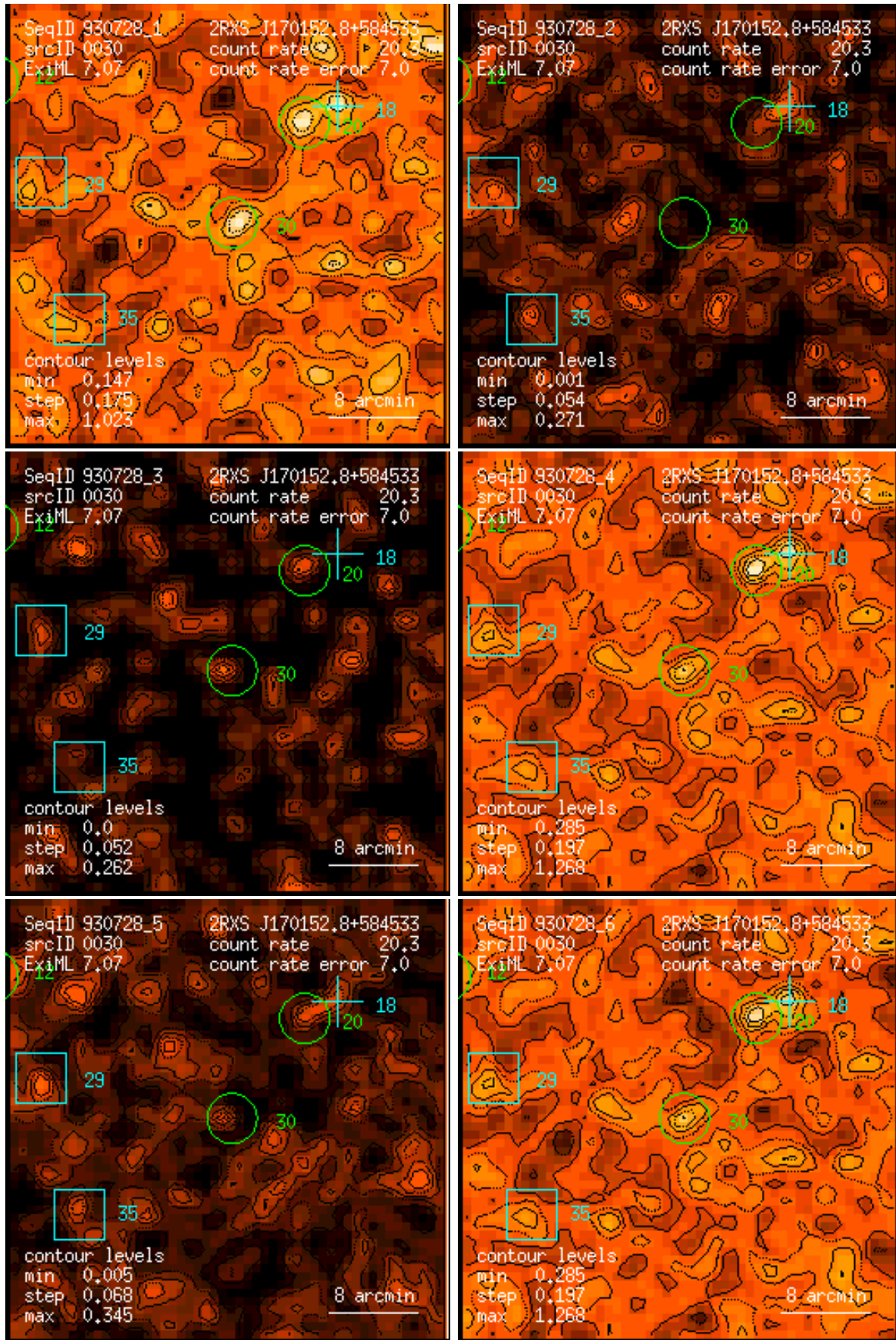
Figure 30: RASS 930728: detection 0030: band rate images, Gaussian filter: (1) PSPC channels 11 – 41, (2) 52 – 90, (3) 91 – 201, (4) 11 – 235, (5) 52 – 201, (6) 11 – 201. Broad band rates in counts/ks. Band rate contour levels in counts/ks/arcmin 2 .
