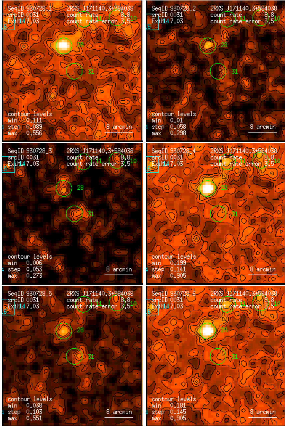
Figure 31: RASS 930728: detection 0031: band rate images, Gaussian filter: (1) PSPC channels 11 – 41, (2) 52 – 90, (3) 91 – 201, (4) 11 – 235, (5) 52 – 201, (6) 11 – 201. Broad band rates in counts/ks. Band rate contour levels in counts/ks/arcmin 2 .
