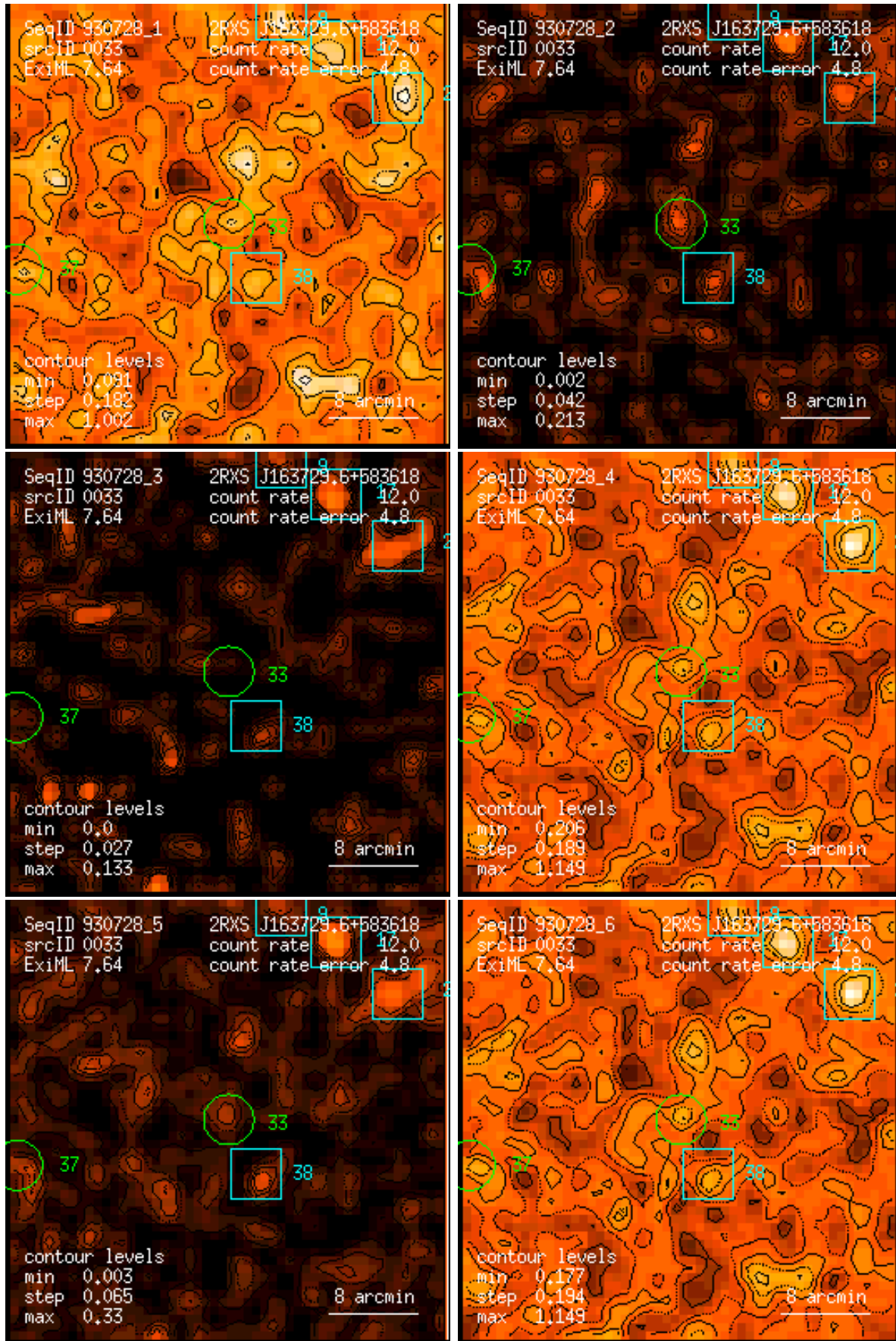
Figure 33: RASS 930728: detection 0033: band rate images, Gaussian filter: (1) PSPC channels 11 – 41, (2) 52 – 90, (3) 91 – 201, (4) 11 – 235, (5) 52 – 201, (6) 11 – 201. Broad band rates in counts/ks. Band rate contour levels in counts/ks/arcmin 2 .
