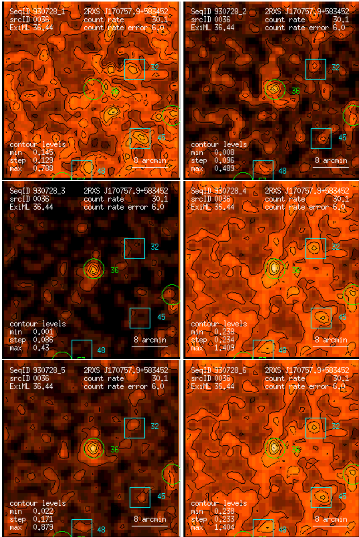
Figure 36: RASS 930728: detection 0036: band rate images, Gaussian filter: (1) PSPC channels 11 – 41, (2) 52 – 90, (3) 91 – 201, (4) 11 – 235, (5) 52 – 201, (6) 11 – 201. Broad band rates in counts/ks. Band rate contour levels in counts/ks/arcmin 2 .
