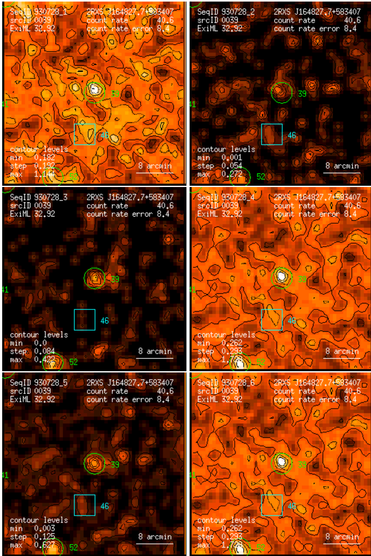
Figure 39: RASS 930728: detection 0039: band rate images, Gaussian filter: (1) PSPC channels 11 – 41, (2) 52 – 90, (3) 91 – 201, (4) 11 – 235, (5) 52 – 201, (6) 11 – 201. Broad band rates in counts/ks. Band rate contour levels in counts/ks/arcmin 2 .
