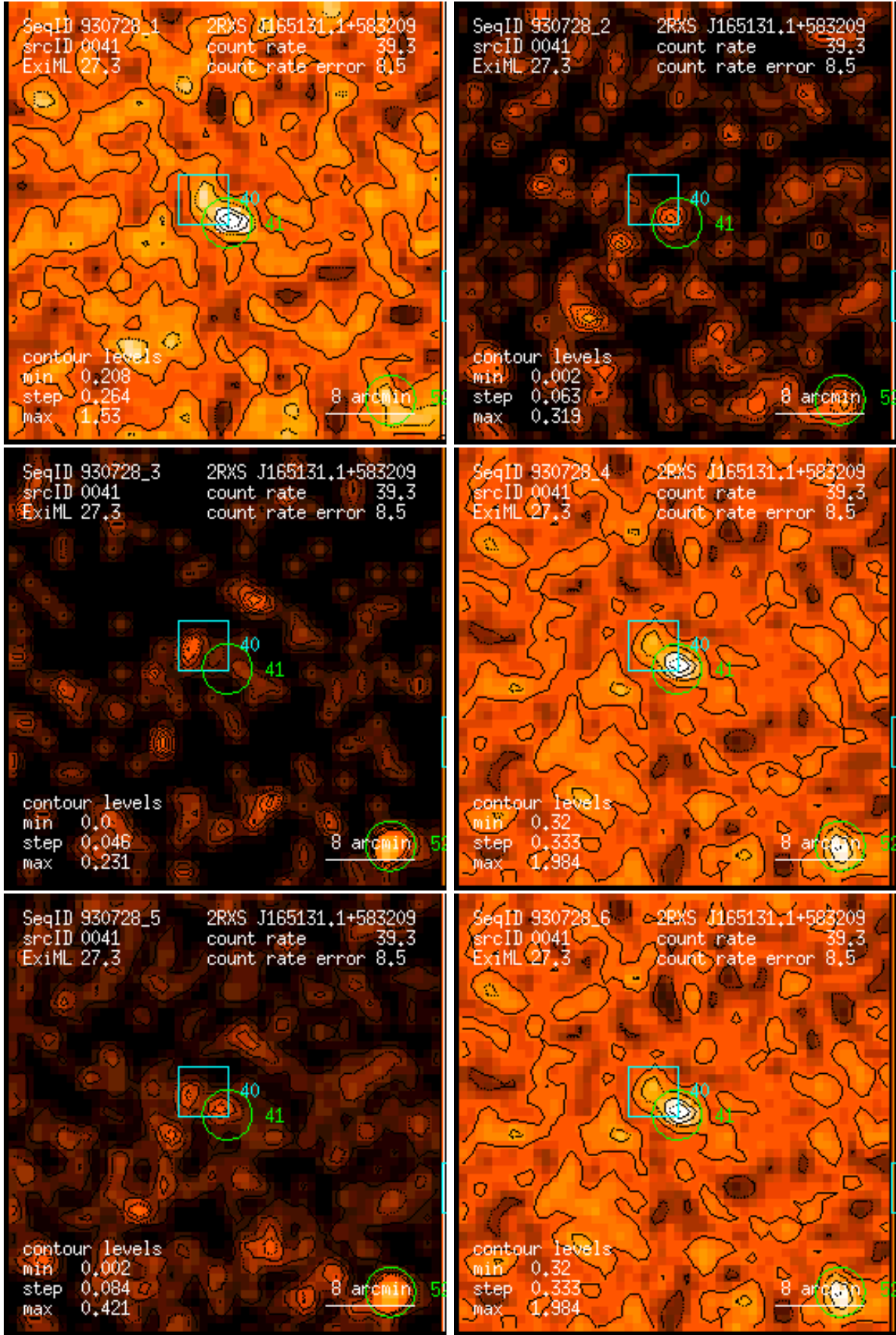
Figure 41: RASS 930728: detection 0041: band rate images, Gaussian filter: (1) PSPC channels 11 – 41, (2) 52 – 90, (3) 91 – 201, (4) 11 – 235, (5) 52 – 201, (6) 11 – 201. Broad band rates in counts/ks. Band rate contour levels in counts/ks/arcmin 2 .
