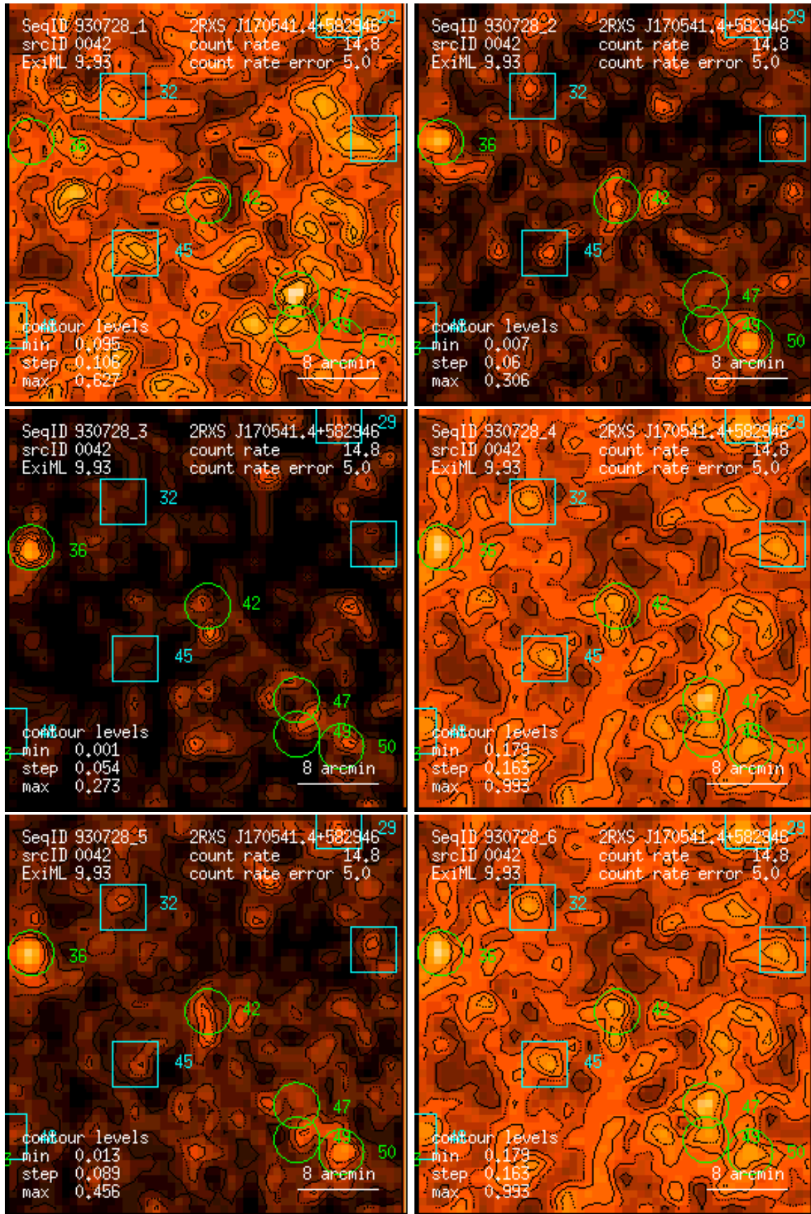
Figure 42: RASS 930728: detection 0042: band rate images, Gaussian filter: (1) PSPC channels 11 – 41, (2) 52 – 90, (3) 91 – 201, (4) 11 – 235, (5) 52 – 201, (6) 11 – 201. Broad band rates in counts/ks. Band rate contour levels in counts/ks/arcmin 2 .
