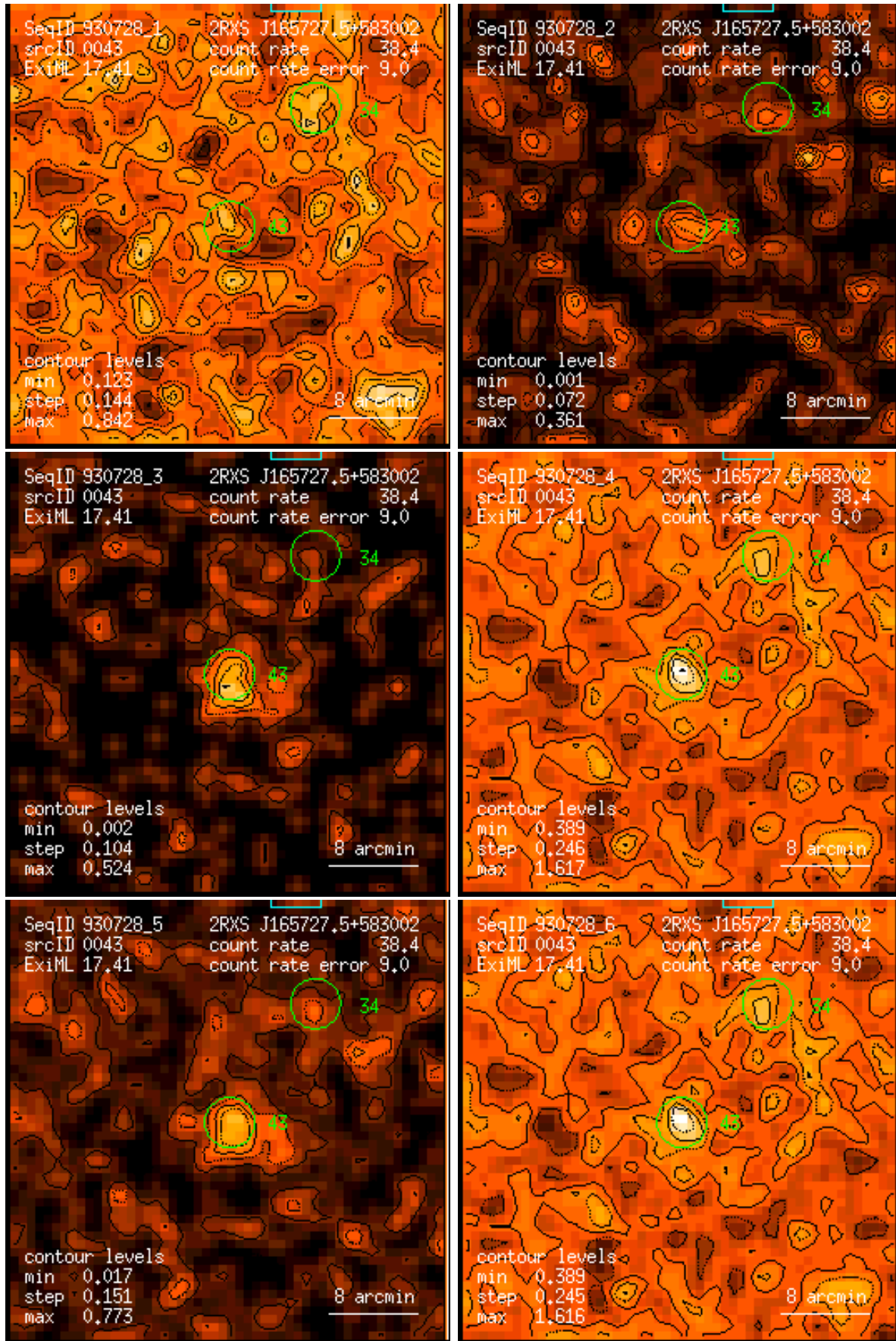
Figure 43: RASS 930728: detection 0043: band rate images, Gaussian filter: (1) PSPC channels 11 – 41, (2) 52 – 90, (3) 91 – 201, (4) 11 – 235, (5) 52 – 201, (6) 11 – 201. Broad band rates in counts/ks. Band rate contour levels in counts/ks/arcmin 2 .
