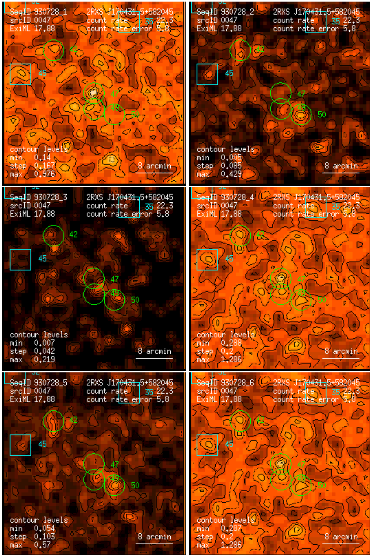
Figure 47: RASS 930728: detection 0047: band rate images, Gaussian filter: (1) PSPC channels 11 – 41, (2) 52 – 90, (3) 91 – 201, (4) 11 – 235, (5) 52 – 201, (6) 11 – 201. Broad band rates in counts/ks. Band rate contour levels in counts/ks/arcmin 2 .
