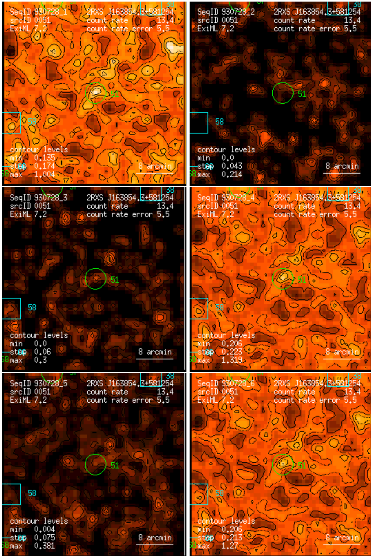
Figure 51: RASS 930728: detection 0051: band rate images, Gaussian filter: (1) PSPC channels 11 – 41, (2) 52 – 90, (3) 91 – 201, (4) 11 – 235, (5) 52 – 201, (6) 11 – 201. Broad band rates in counts/ks. Band rate contour levels in counts/ks/arcmin 2 .
