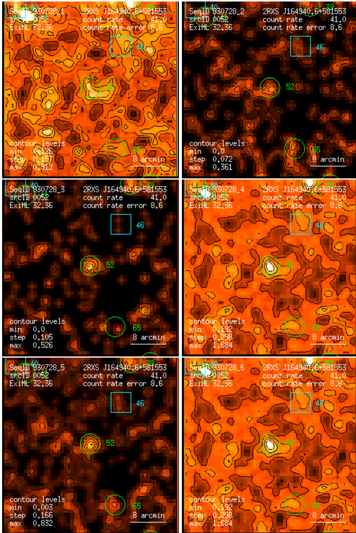
Figure 52: RASS 930728: detection 0052: band rate images, Gaussian filter: (1) PSPC channels 11 – 41, (2) 52 – 90, (3) 91 – 201, (4) 11 – 235, (5) 52 – 201, (6) 11 – 201. Broad band rates in counts/ks. Band rate contour levels in counts/ks/arcmin 2 .
