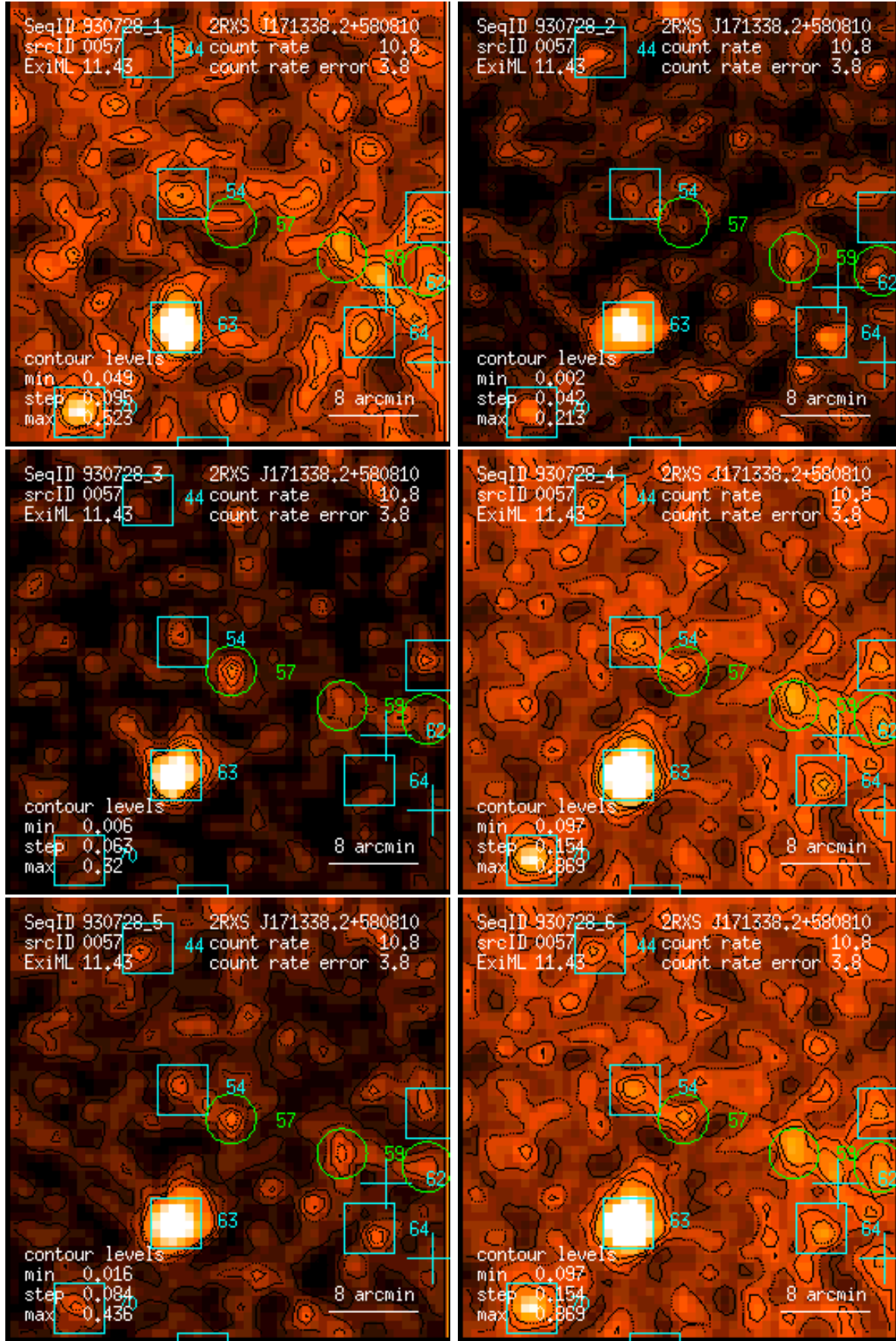
Figure 57: RASS 930728: detection 0057: band rate images, Gaussian filter: (1) PSPC channels 11 – 41, (2) 52 – 90, (3) 91 – 201, (4) 11 – 235, (5) 52 – 201, (6) 11 – 201. Broad band rates in counts/ks. Band rate contour levels in counts/ks/arcmin 2 .
