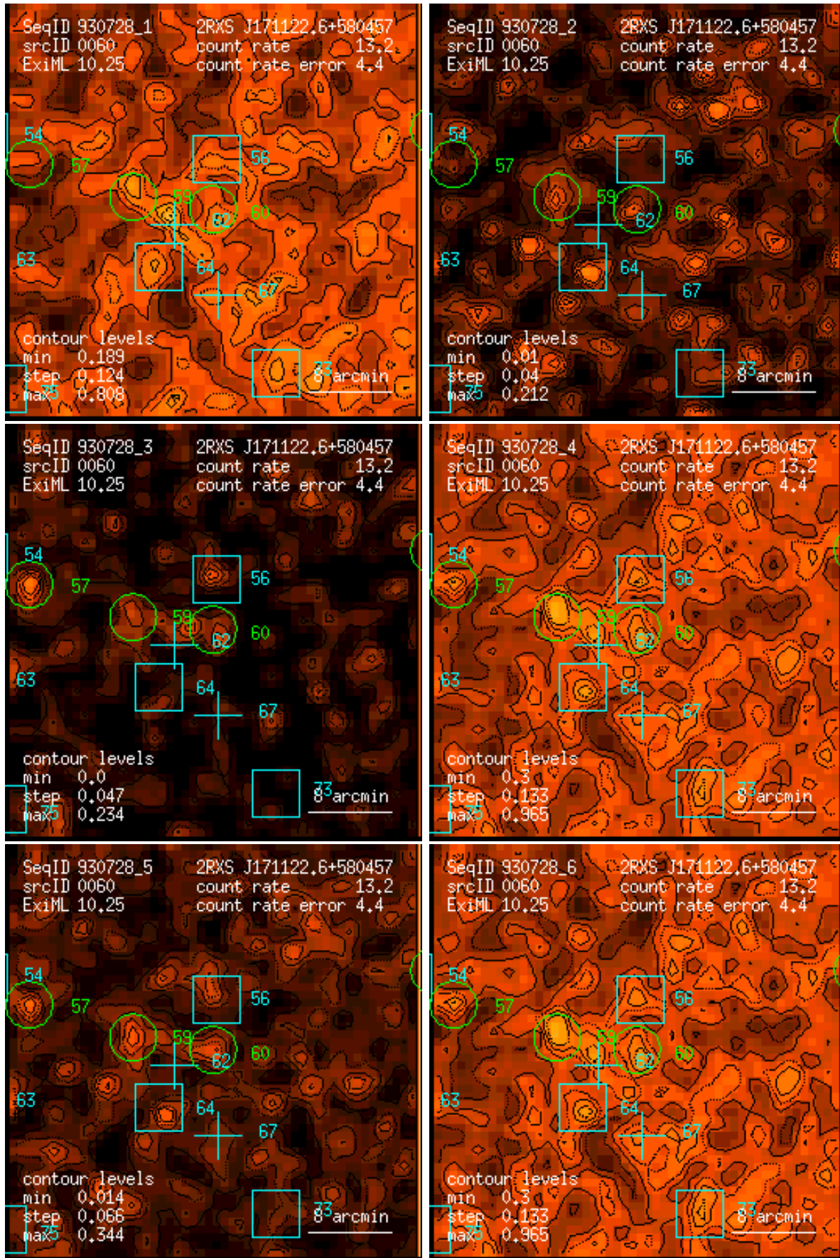
Figure 60: RASS 930728: detection 0060: band rate images, Gaussian filter: (1) PSPC channels 11 – 41, (2) 52 – 90, (3) 91 – 201, (4) 11 – 235, (5) 52 – 201, (6) 11 – 201. Broad band rates in counts/ks. Band rate contour levels in counts/ks/arcmin 2 .
