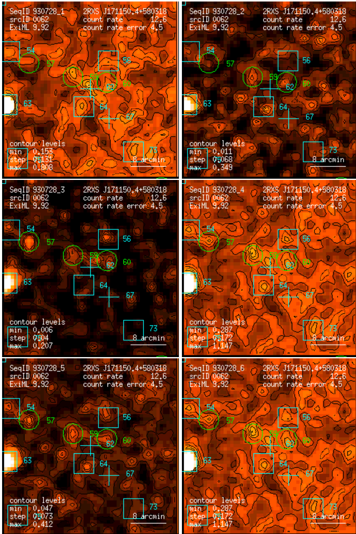
Figure 62: RASS 930728: detection 0062: band rate images, Gaussian filter: (1) PSPC channels 11 – 41, (2) 52 – 90, (3) 91 – 201, (4) 11 – 235, (5) 52 – 201, (6) 11 – 201. Broad band rates in counts/ks. Band rate contour levels in counts/ks/arcmin 2 .
