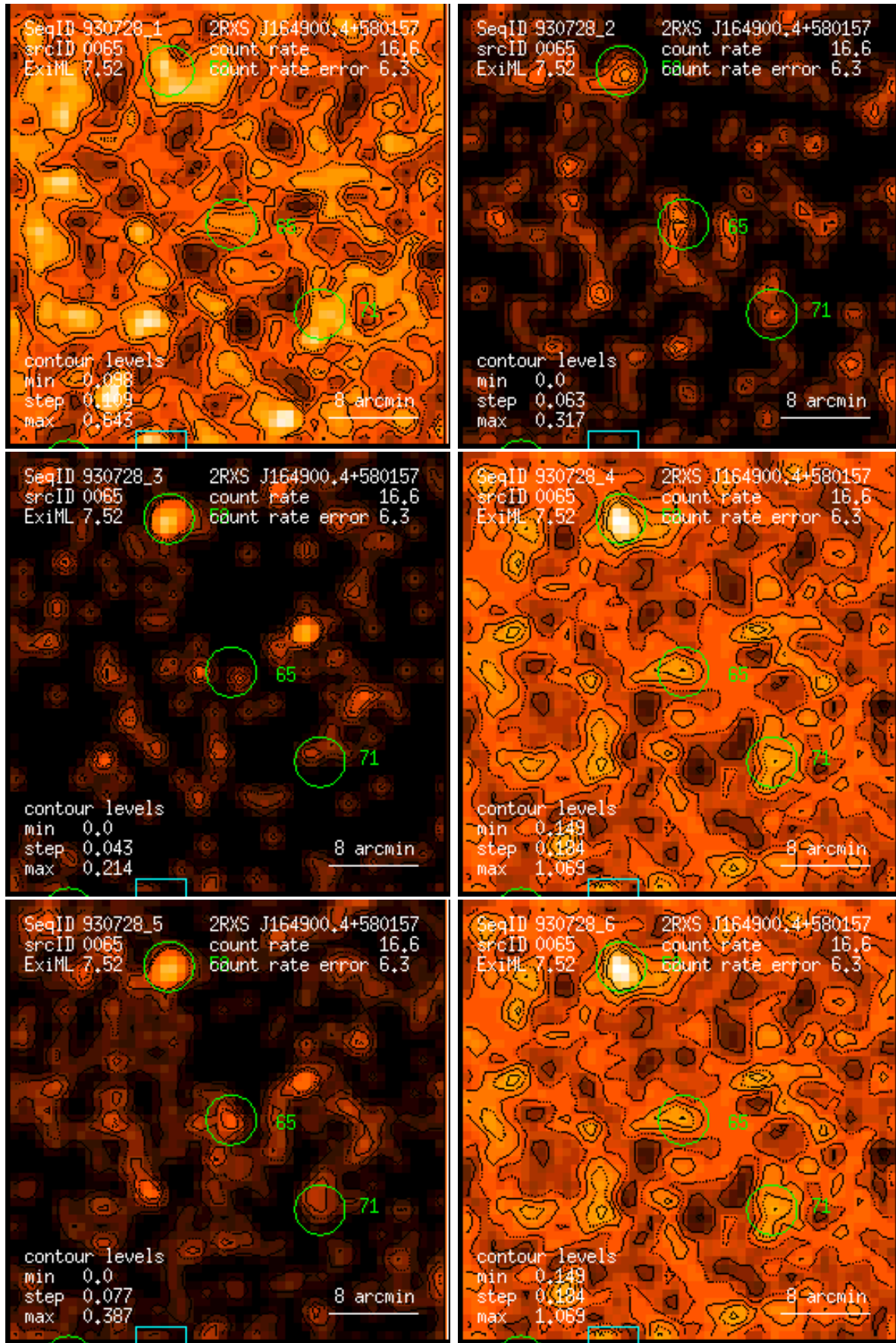
Figure 65: RASS 930728: detection 0065: band rate images, Gaussian filter: (1) PSPC channels 11 – 41, (2) 52 – 90, (3) 91 – 201, (4) 11 – 235, (5) 52 – 201, (6) 11 – 201. Broad band rates in counts/ks. Band rate contour levels in counts/ks/arcmin 2 .
