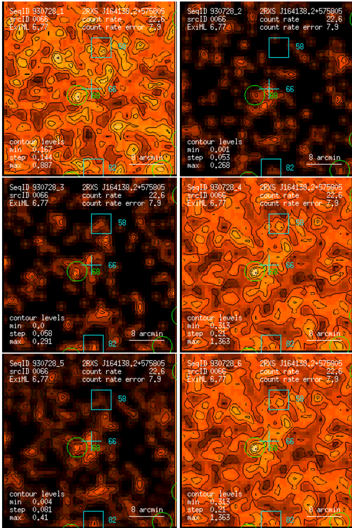
Figure 66: RASS 930728: detection 0066: band rate images, Gaussian filter: (1) PSPC channels 11 – 41, (2) 52 – 90, (3) 91 – 201, (4) 11 – 235, (5) 52 – 201, (6) 11 – 201. Broad band rates in counts/ks. Band rate contour levels in counts/ks/arcmin 2 .
