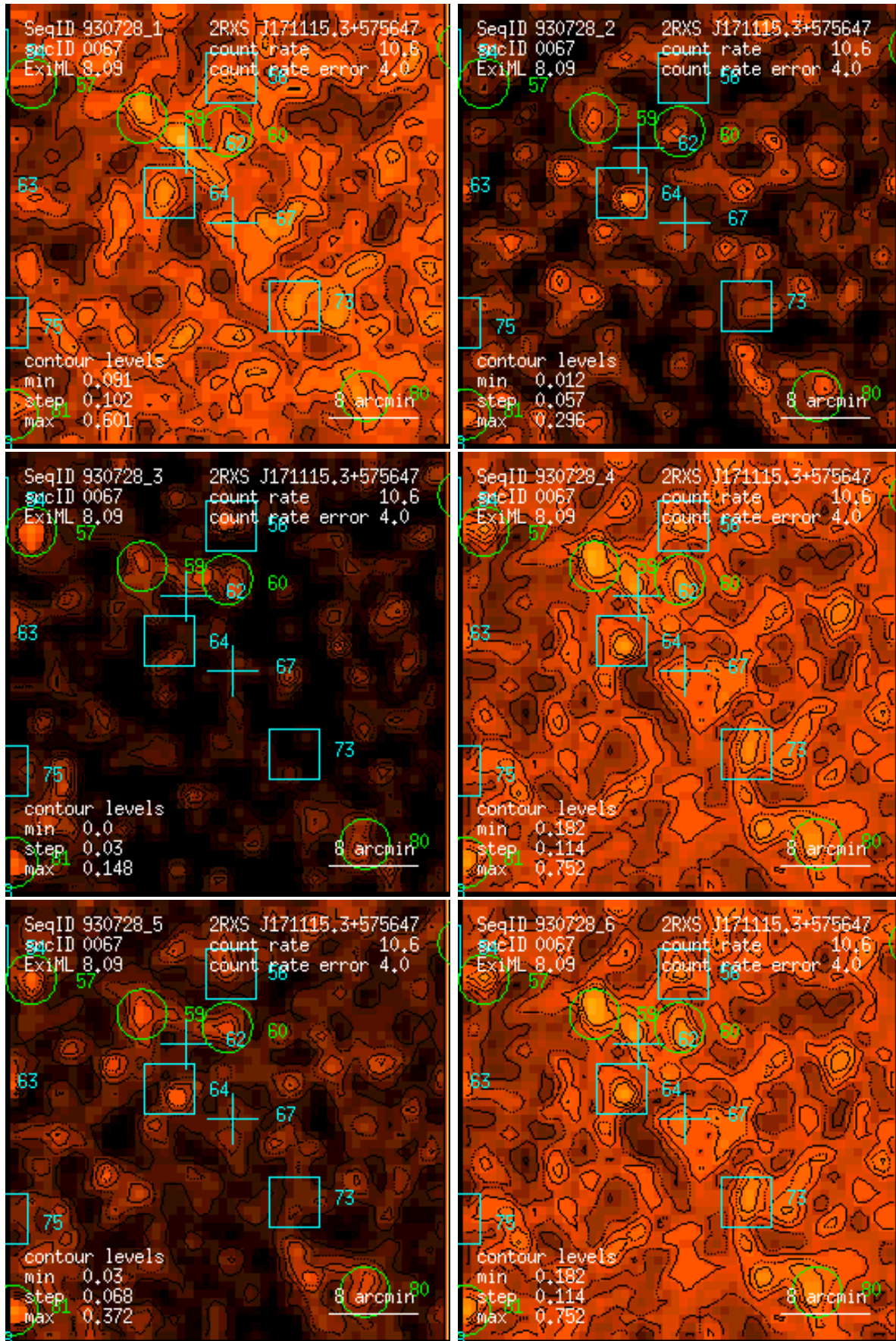
Figure 67: RASS 930728: detection 0067: band rate images, Gaussian filter: (1) PSPC channels 11 – 41, (2) 52 – 90, (3) 91 – 201, (4) 11 – 235, (5) 52 – 201, (6) 11 – 201. Broad band rates in counts/ks. Band rate contour levels in counts/ks/arcmin 2 .
