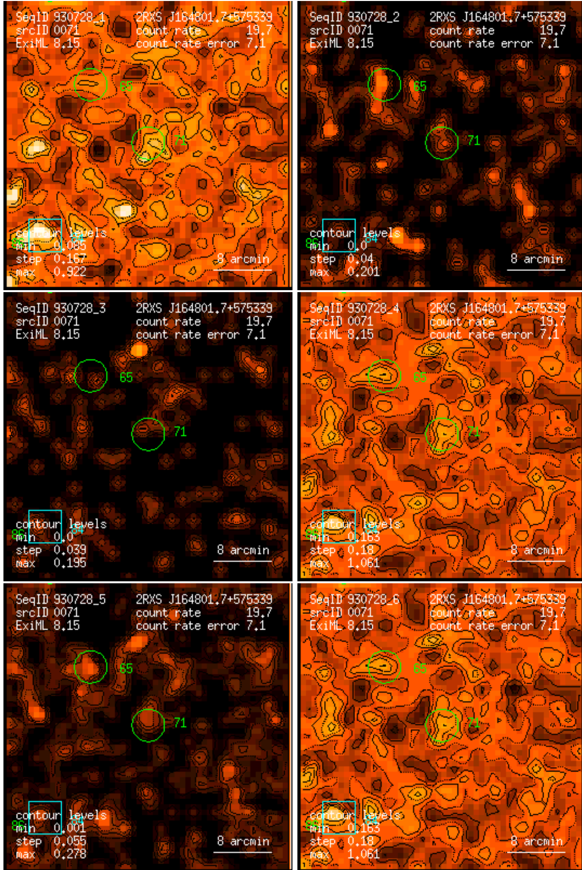
Figure 71: RASS 930728: detection 0071: band rate images, Gaussian filter: (1) PSPC channels 11 – 41, (2) 52 – 90, (3) 91 – 201, (4) 11 – 235, (5) 52 – 201, (6) 11 – 201. Broad band rates in counts/ks. Band rate contour levels in counts/ks/arcmin 2 .
