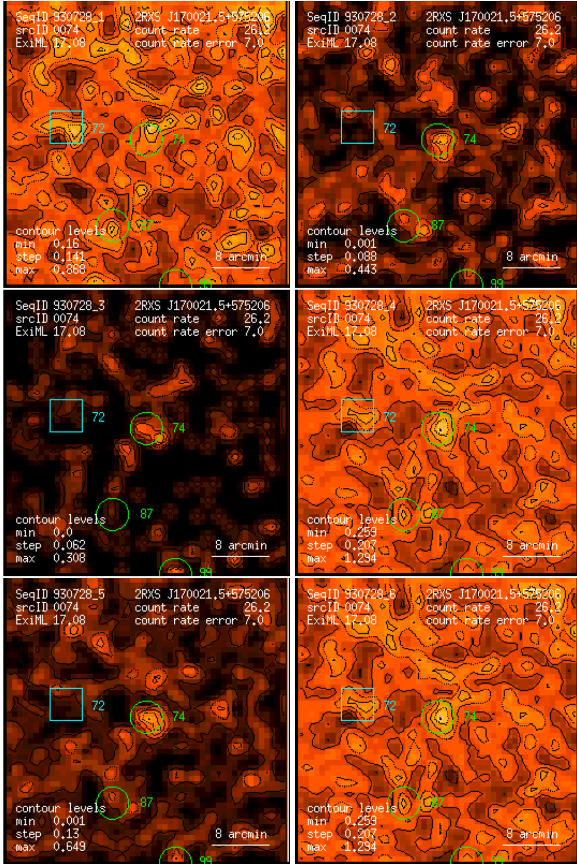
Figure 74: RASS 930728: detection 0074: band rate images, Gaussian filter: (1) PSPC channels 11 – 41, (2) 52 – 90, (3) 91 – 201, (4) 11 – 235, (5) 52 – 201, (6) 11 – 201. Broad band rates in counts/ks. Band rate contour levels in counts/ks/arcmin 2 .
