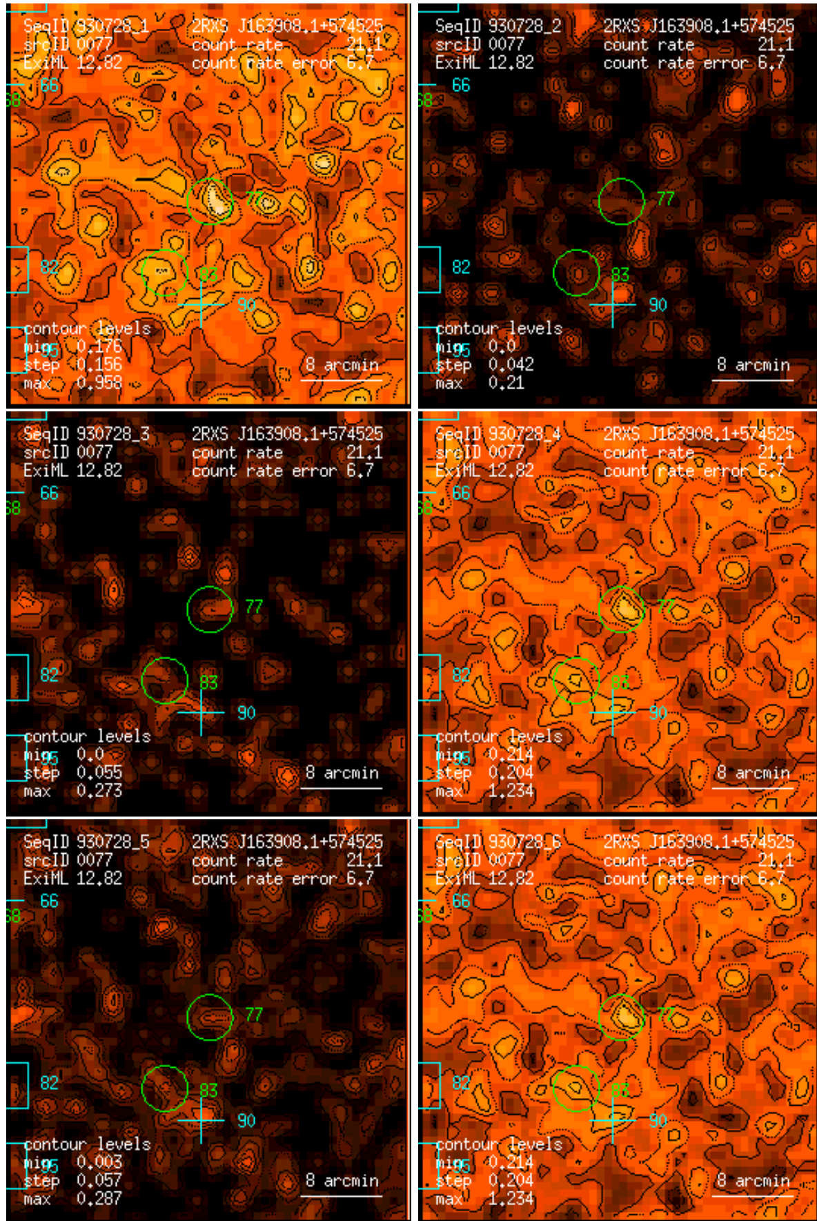
Figure 77: RASS 930728: detection 0077: band rate images, Gaussian filter: (1) PSPC channels 11 – 41, (2) 52 – 90, (3) 91 – 201, (4) 11 – 235, (5) 52 – 201, (6) 11 – 201. Broad band rates in counts/ks. Band rate contour levels in counts/ks/arcmin 2 .
