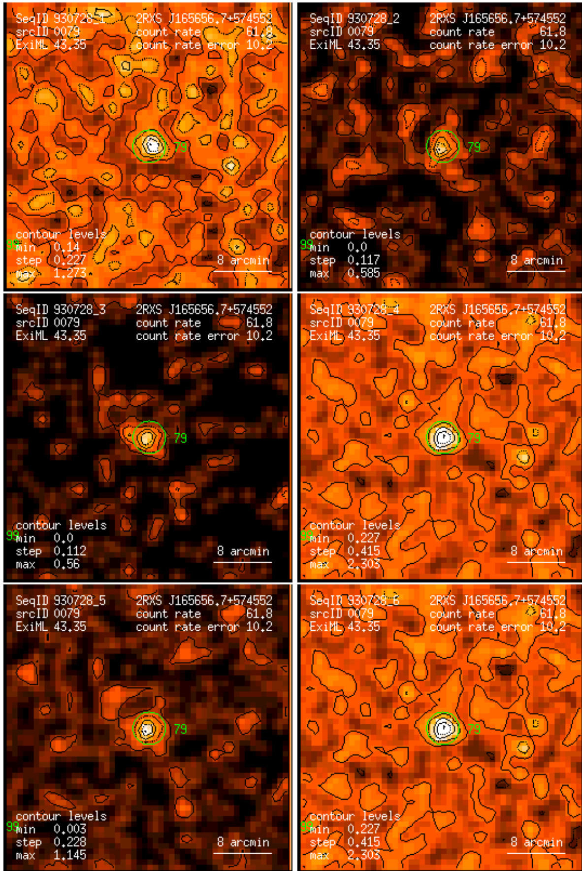
Figure 79: RASS 930728: detection 0079: band rate images, Gaussian filter: (1) PSPC channels 11 – 41, (2) 52 – 90, (3) 91 – 201, (4) 11 – 235, (5) 52 – 201, (6) 11 – 201. Broad band rates in counts/ks. Band rate contour levels in counts/ks/arcmin 2 .
