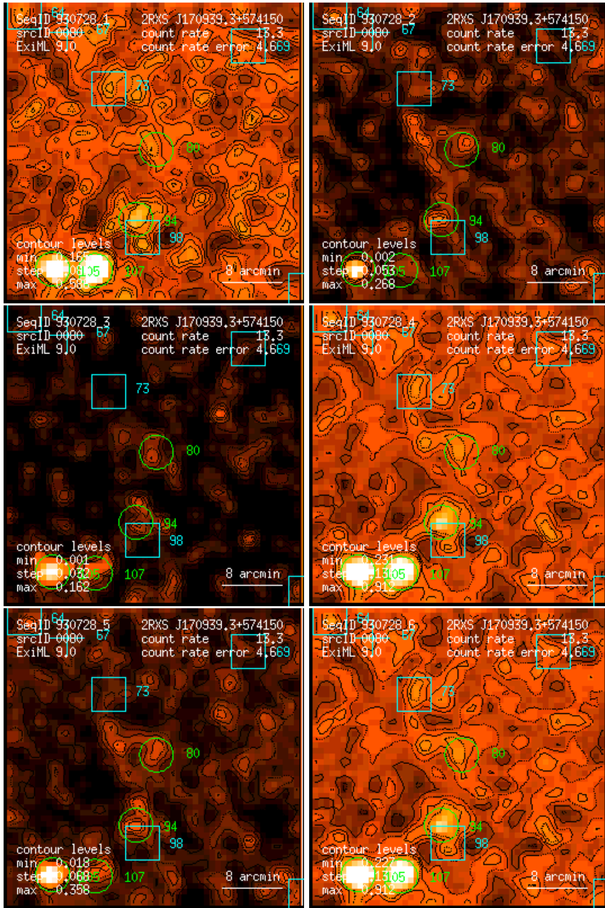
Figure 80: RASS 930728: detection 0080: band rate images, Gaussian filter: (1) PSPC channels 11 – 41, (2) 52 – 90, (3) 91 – 201, (4) 11 – 235, (5) 52 – 201, (6) 11 – 201. Broad band rates in counts/ks. Band rate contour levels in counts/ks/arcmin 2 .
