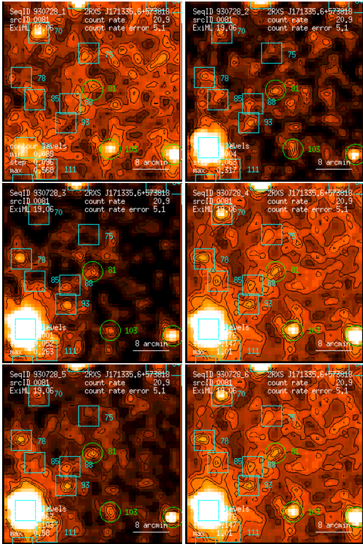
Figure 81: RASS 930728: detection 0081: band rate images, Gaussian filter: (1) PSPC channels 11 – 41, (2) 52 – 90, (3) 91 – 201, (4) 11 – 235, (5) 52 – 201, (6) 11 – 201. Broad band rates in counts/ks. Band rate contour levels in counts/ks/arcmin 2 .
