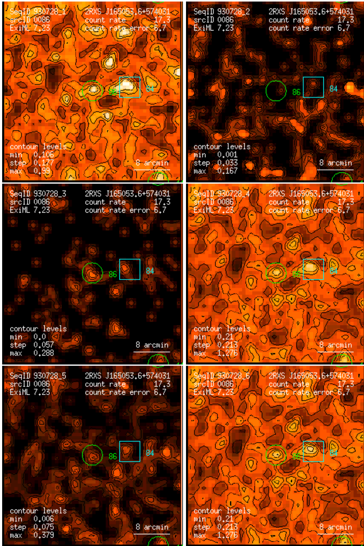
Figure 86: RASS 930728: detection 0086: band rate images, Gaussian filter: (1) PSPC channels 11 – 41, (2) 52 – 90, (3) 91 – 201, (4) 11 – 235, (5) 52 – 201, (6) 11 – 201. Broad band rates in counts/ks. Band rate contour levels in counts/ks/arcmin 2 .
