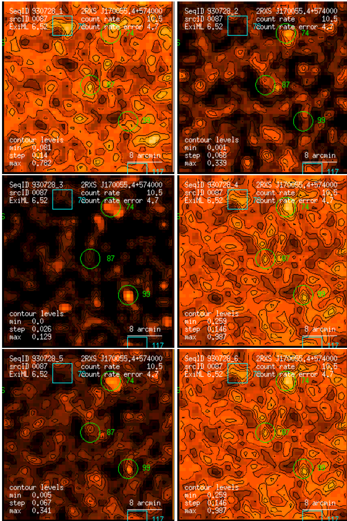
Figure 87: RASS 930728: detection 0087: band rate images, Gaussian filter: (1) PSPC channels 11 – 41, (2) 52 – 90, (3) 91 – 201, (4) 11 – 235, (5) 52 – 201, (6) 11 – 201. Broad band rates in counts/ks. Band rate contour levels in counts/ks/arcmin 2 .
