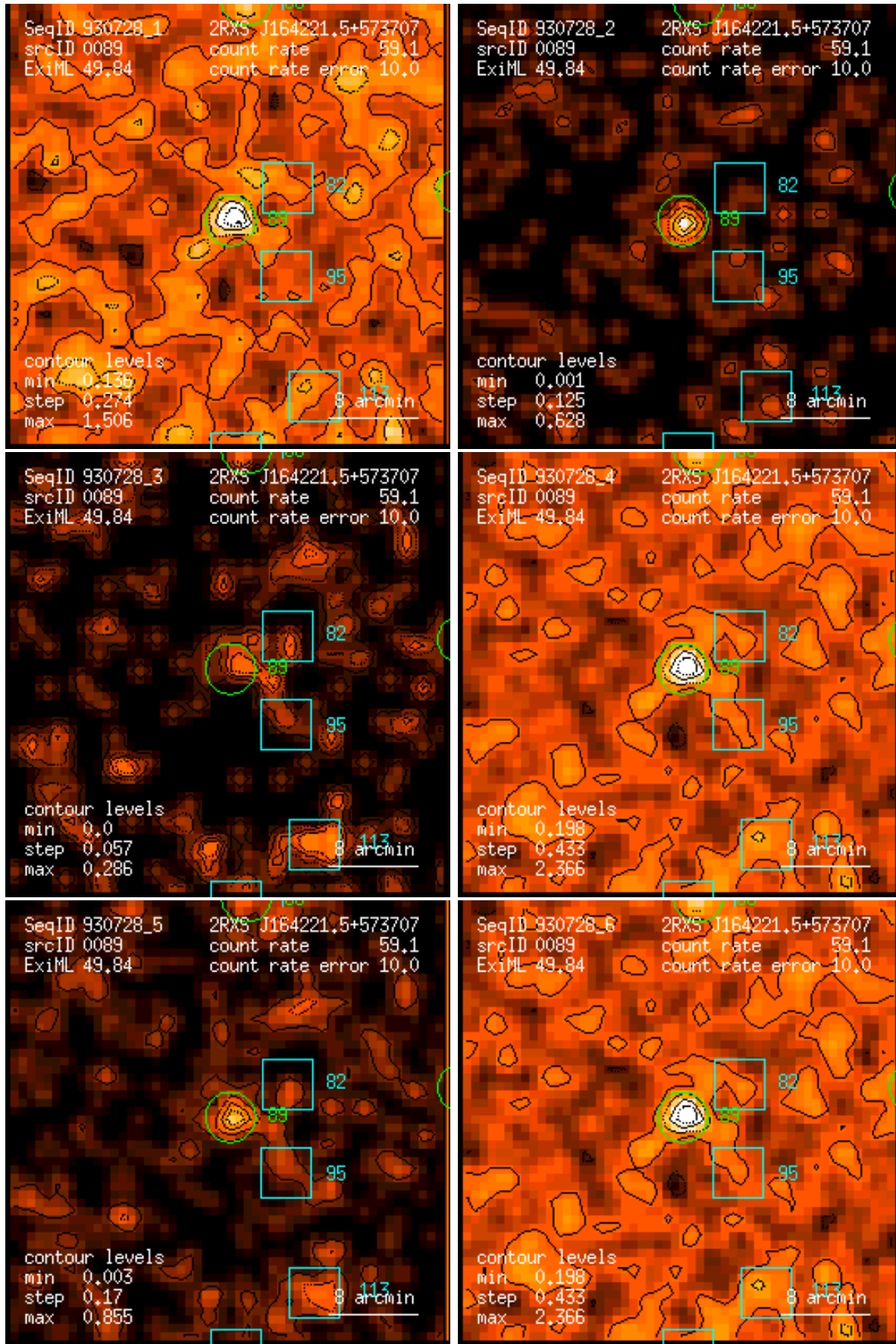
Figure 89: RASS 930728: detection 0089: band rate images, Gaussian filter: (1) PSPC channels 11 – 41, (2) 52 – 90, (3) 91 – 201, (4) 11 – 235, (5) 52 – 201, (6) 11 – 201. Broad band rates in counts/ks. Band rate contour levels in counts/ks/arcmin 2 .
