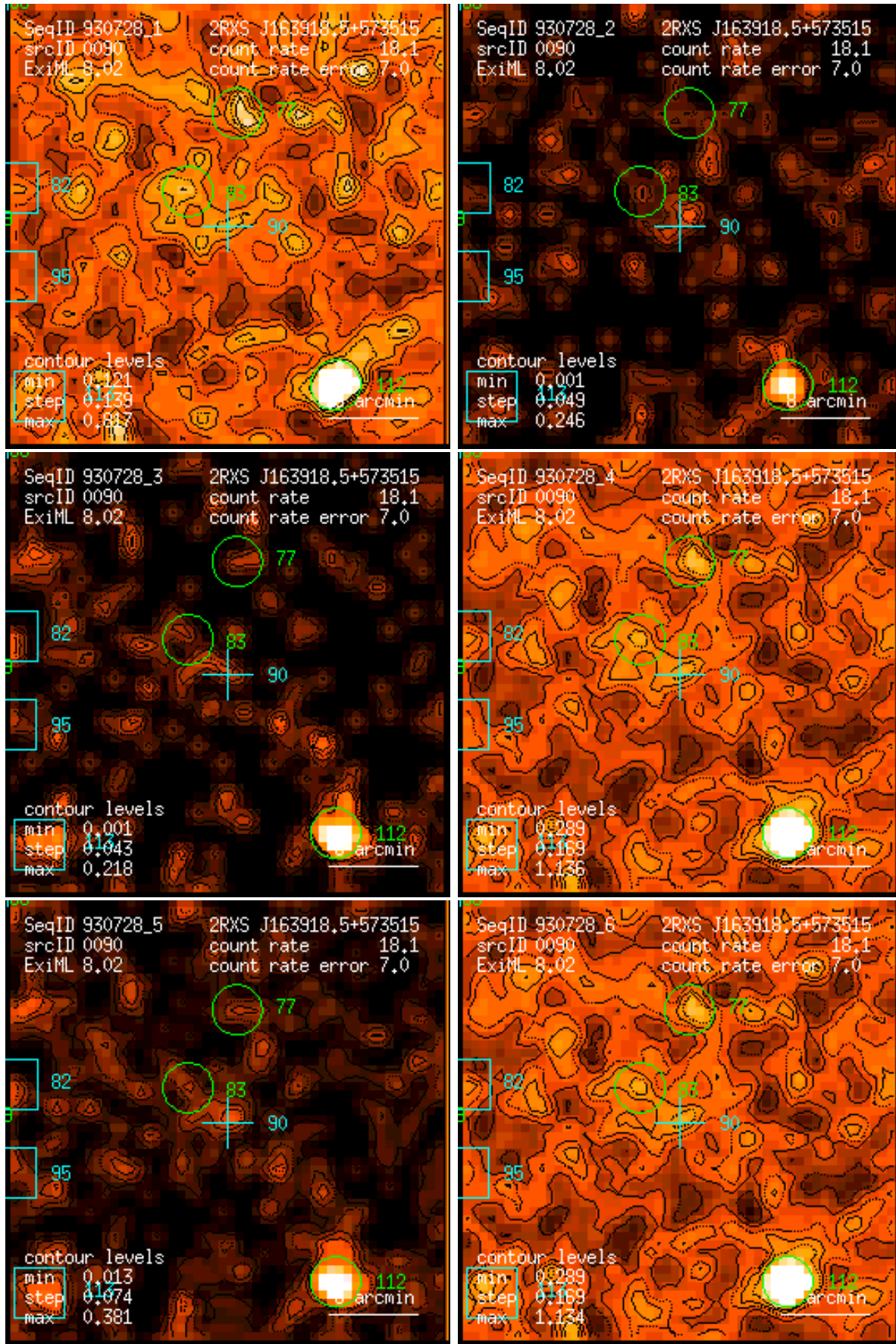
Figure 90: RASS 930728: detection 0090: band rate images, Gaussian filter: (1) PSPC channels 11 – 41, (2) 52 – 90, (3) 91 – 201, (4) 11 – 235, (5) 52 – 201, (6) 11 – 201. Broad band rates in counts/ks. Band rate contour levels in counts/ks/arcmin 2 .
