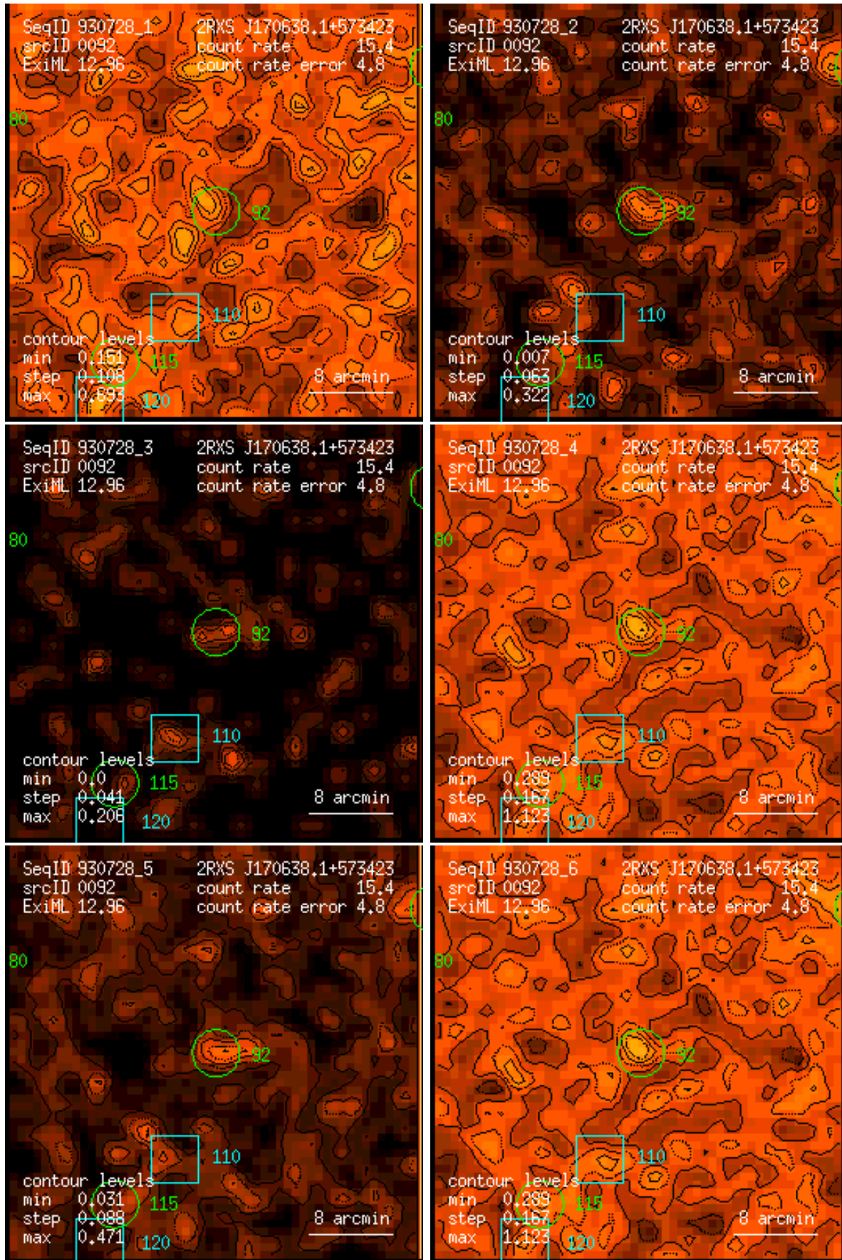
Figure 92: RASS 930728: detection 0092: band rate images, Gaussian filter: (1) PSPC channels 11 – 41, (2) 52 – 90, (3) 91 – 201, (4) 11 – 235, (5) 52 – 201, (6) 11 – 201. Broad band rates in counts/ks. Band rate contour levels in counts/ks/arcmin 2 .
