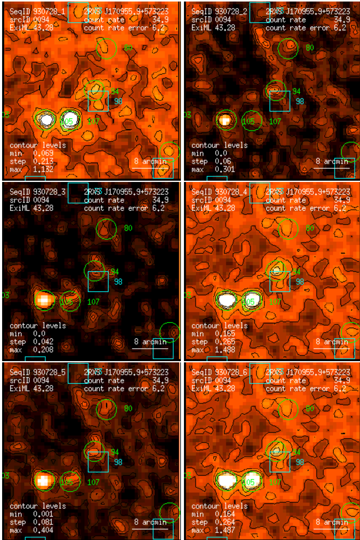
Figure 94: RASS 930728: detection 0094: band rate images, Gaussian filter: (1) PSPC channels 11 – 41, (2) 52 – 90, (3) 91 – 201, (4) 11 – 235, (5) 52 – 201, (6) 11 – 201. Broad band rates in counts/ks. Band rate contour levels in counts/ks/arcmin 2 .
