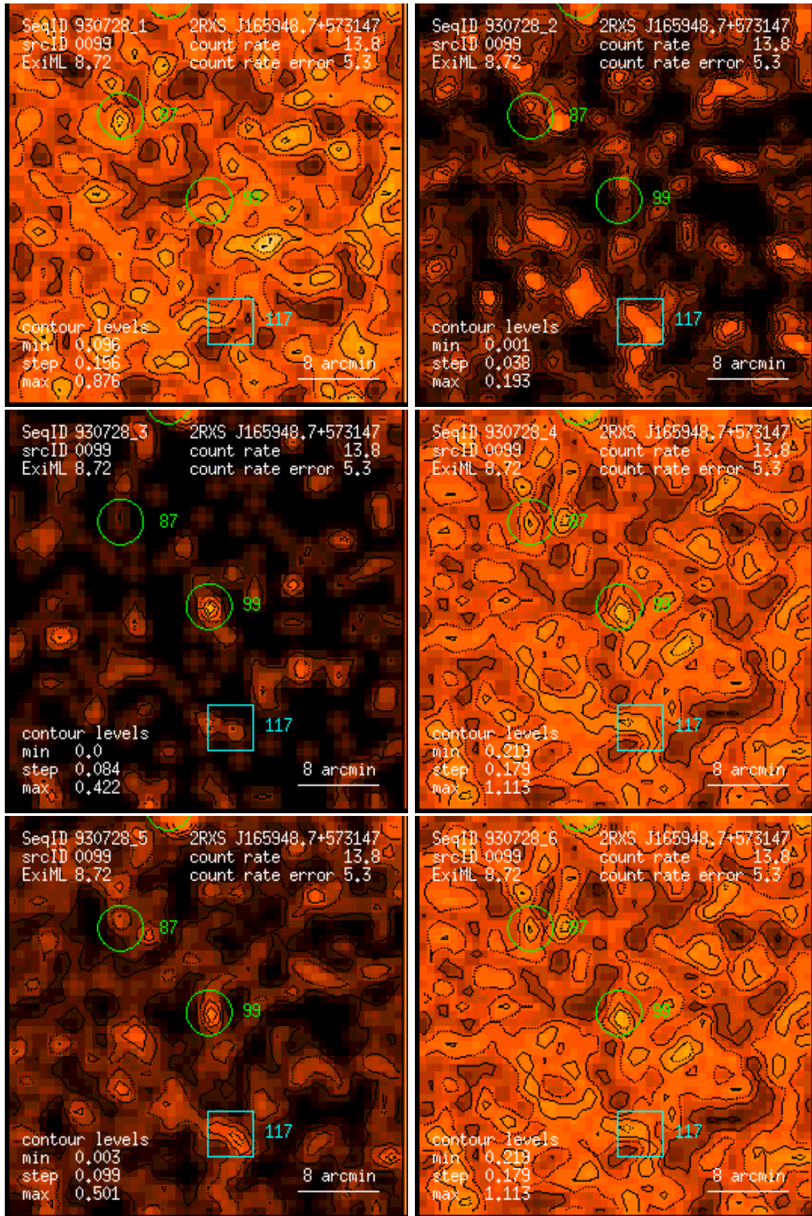
Figure 99: RASS 930728: detection 0099: band rate images, Gaussian filter: (1) PSPC channels 11 – 41, (2) 52 – 90, (3) 91 – 201, (4) 11 – 235, (5) 52 – 201, (6) 11 – 201. Broad band rates in counts/ks. Band rate contour levels in counts/ks/arcmin 2 .
