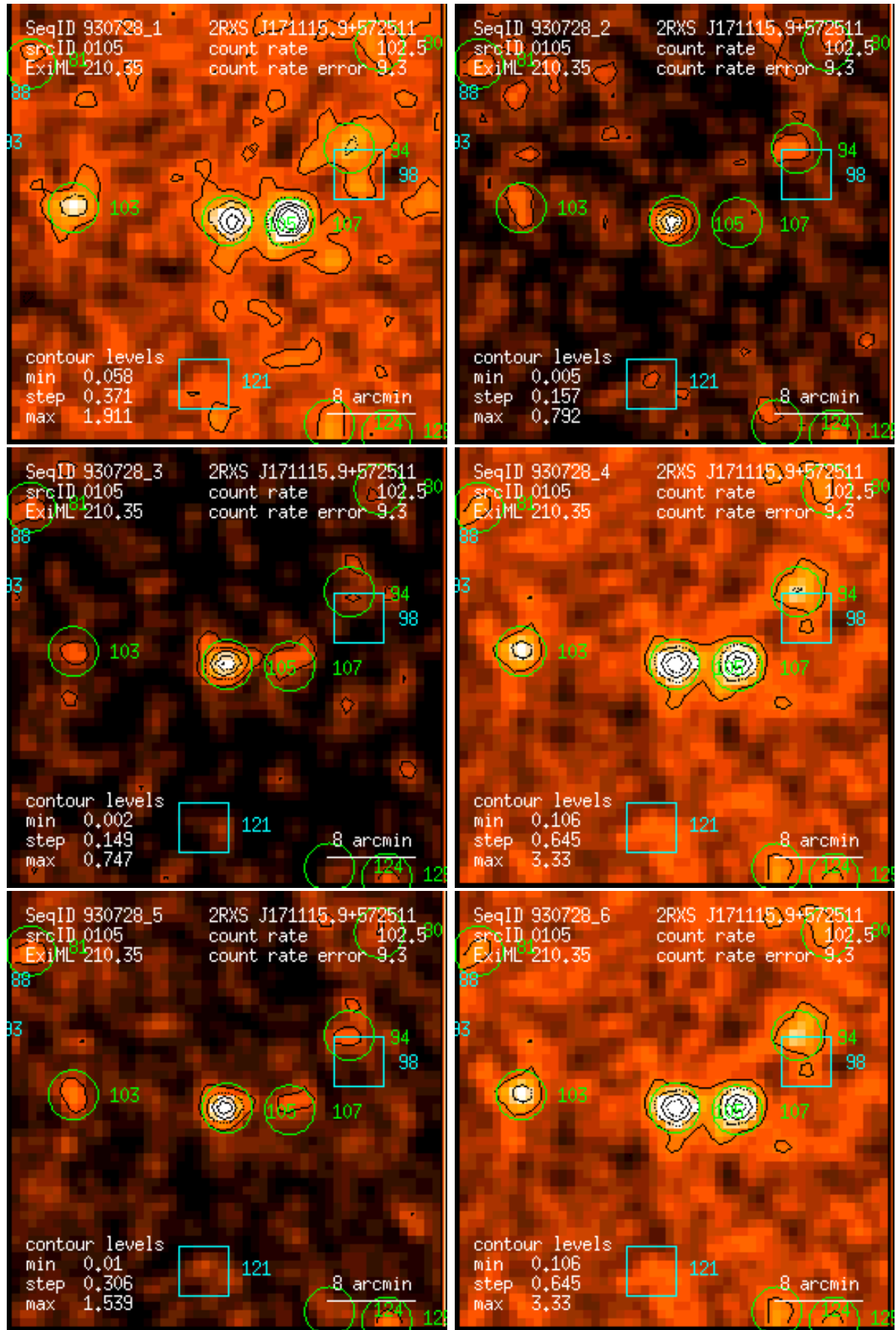
Figure 105: RASS 930728: detection 0105: band rate images, Gaussian filter: (1) PSPC channels 11 – 41, (2) 52 – 90, (3) 91 – 201, (4) 11 – 235, (5) 52 – 201, (6) 11 – 201. Broad band rates in counts/ks. Band rate contour levels in counts/ks/arcmin 2 .
