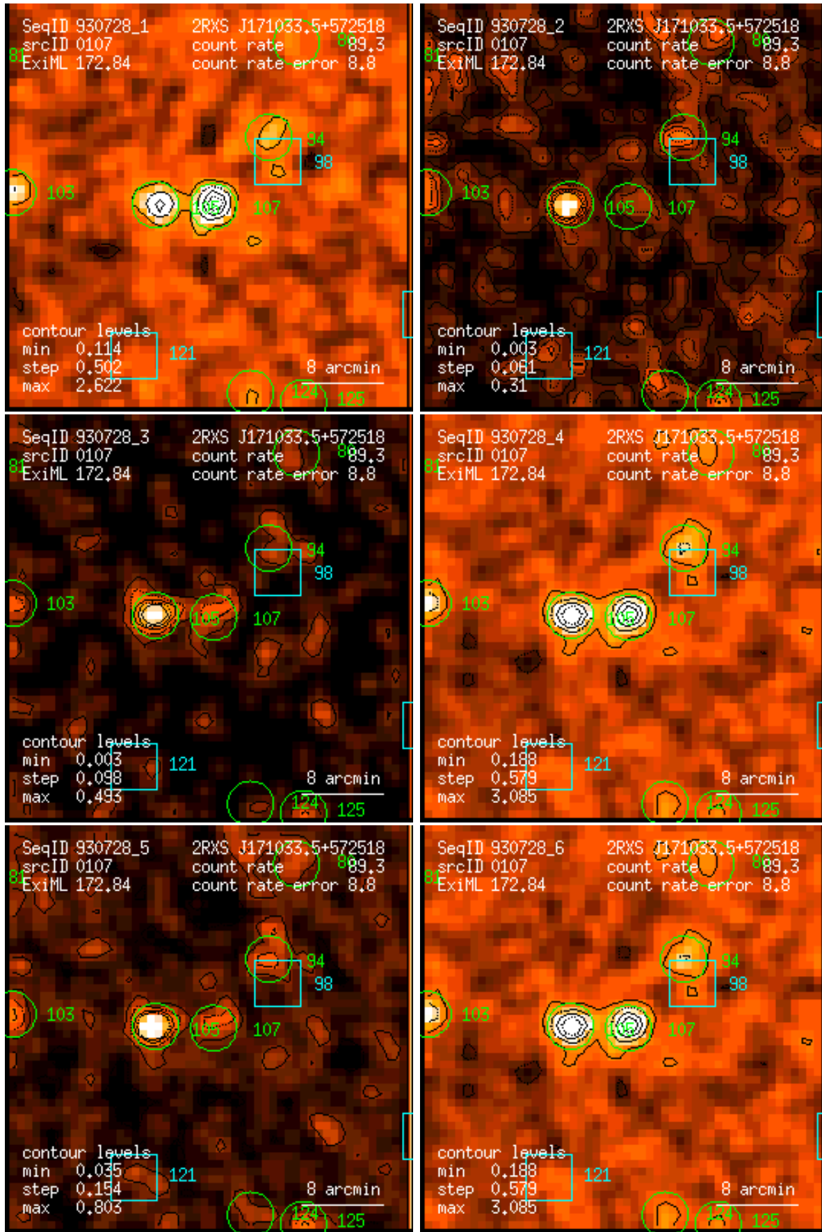
Figure 107: RASS 930728: detection 0107: band rate images, Gaussian filter: (1) PSPC channels 11 – 41, (2) 52 – 90, (3) 91 – 201, (4) 11 – 235, (5) 52 – 201, (6) 11 – 201. Broad band rates in counts/ks. Band rate contour levels in counts/ks/arcmin 2 .
