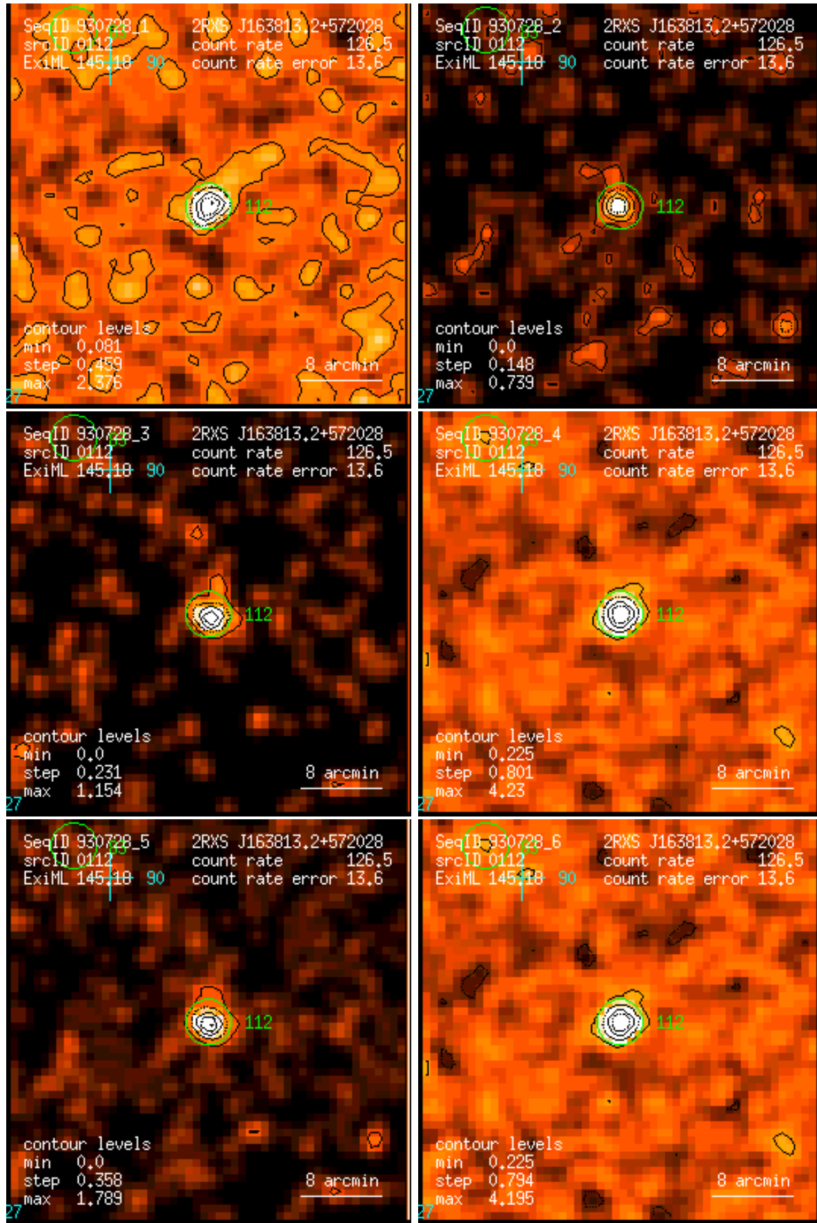
Figure 112: RASS 930728: detection 0112: band rate images, Gaussian filter: (1) PSPC channels 11 – 41, (2) 52 – 90, (3) 91 – 201, (4) 11 – 235, (5) 52 – 201, (6) 11 – 201. Broad band rates in counts/ks. Band rate contour levels in counts/ks/arcmin 2 .
