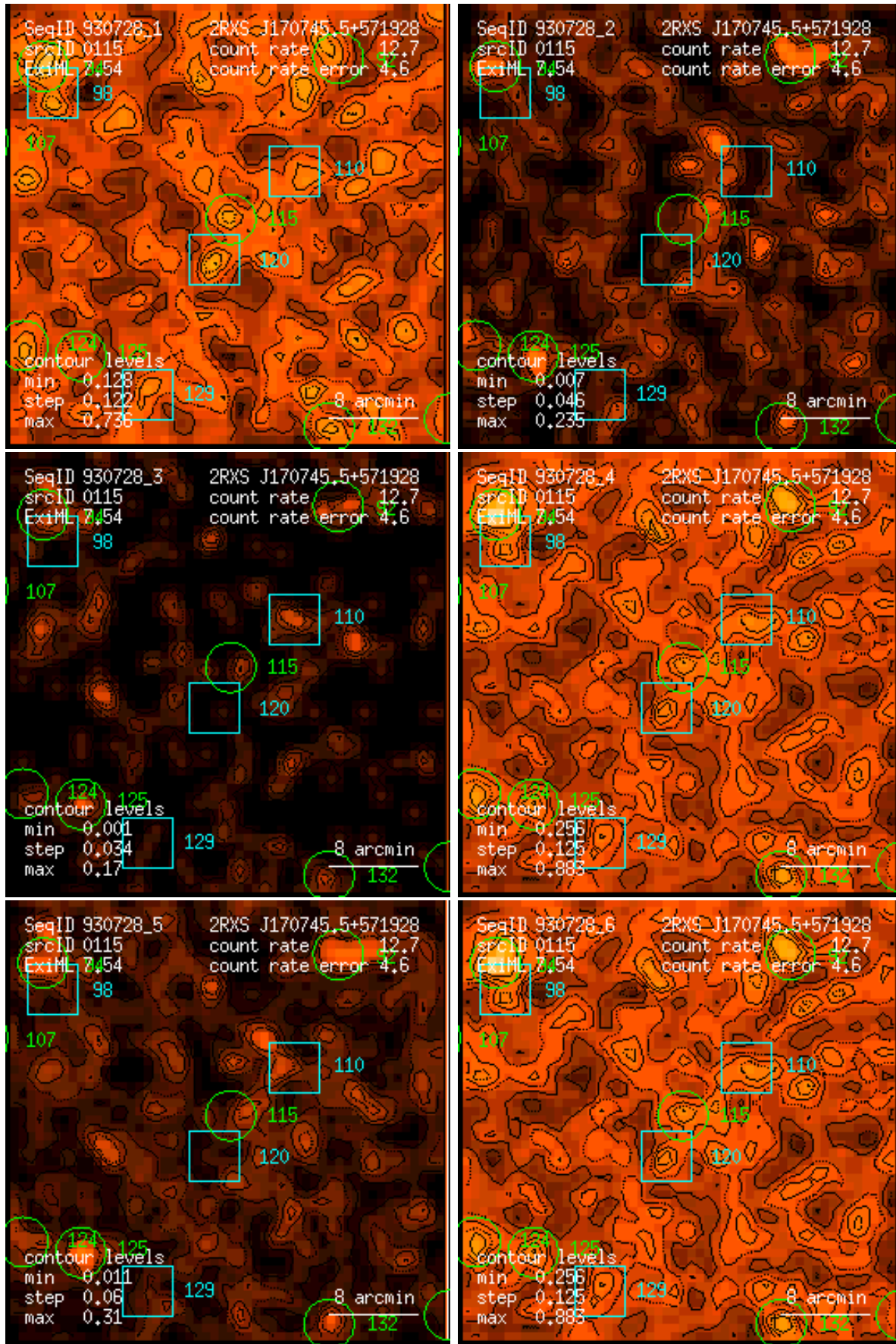
Figure 115: RASS 930728: detection 0115: band rate images, Gaussian filter: (1) PSPC channels 11 – 41, (2) 52 – 90, (3) 91 – 201, (4) 11 – 235, (5) 52 – 201, (6) 11 – 201. Broad band rates in counts/ks. Band rate contour levels in counts/ks/arcmin 2 .
