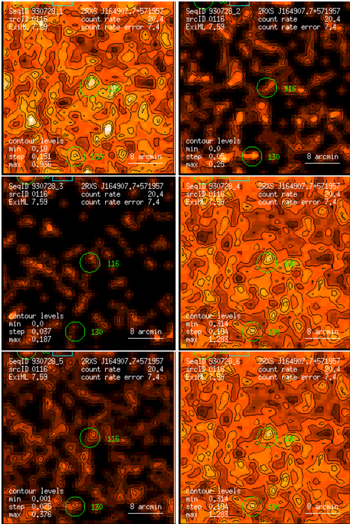
Figure 116: RASS 930728: detection 0116: band rate images, Gaussian filter: (1) PSPC channels 11 – 41, (2) 52 – 90, (3) 91 – 201, (4) 11 – 235, (5) 52 – 201, (6) 11 – 201. Broad band rates in counts/ks. Band rate contour levels in counts/ks/arcmin 2 .
