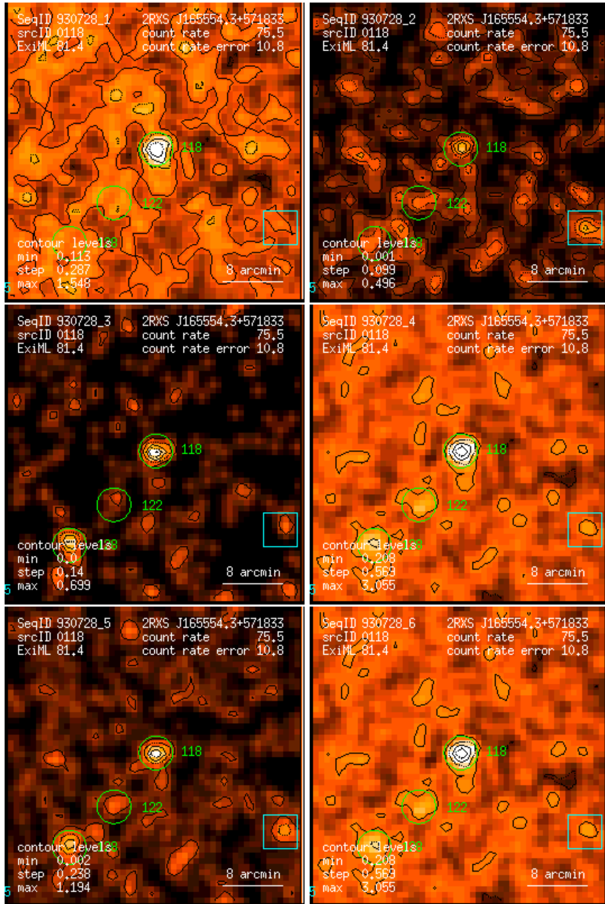
Figure 118: RASS 930728: detection 0118: band rate images, Gaussian filter: (1) PSPC channels 11 – 41, (2) 52 – 90, (3) 91 – 201, (4) 11 – 235, (5) 52 – 201, (6) 11 – 201. Broad band rates in counts/ks. Band rate contour levels in counts/ks/arcmin 2 .
