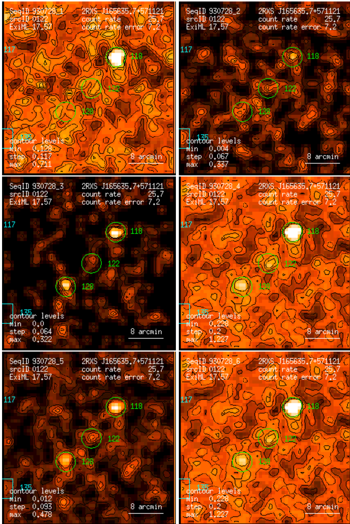
Figure 122: RASS 930728: detection 0122: band rate images, Gaussian filter: (1) PSPC channels 11 – 41, (2) 52 – 90, (3) 91 – 201, (4) 11 – 235, (5) 52 – 201, (6) 11 – 201. Broad band rates in counts/ks. Band rate contour levels in counts/ks/arcmin 2 .
