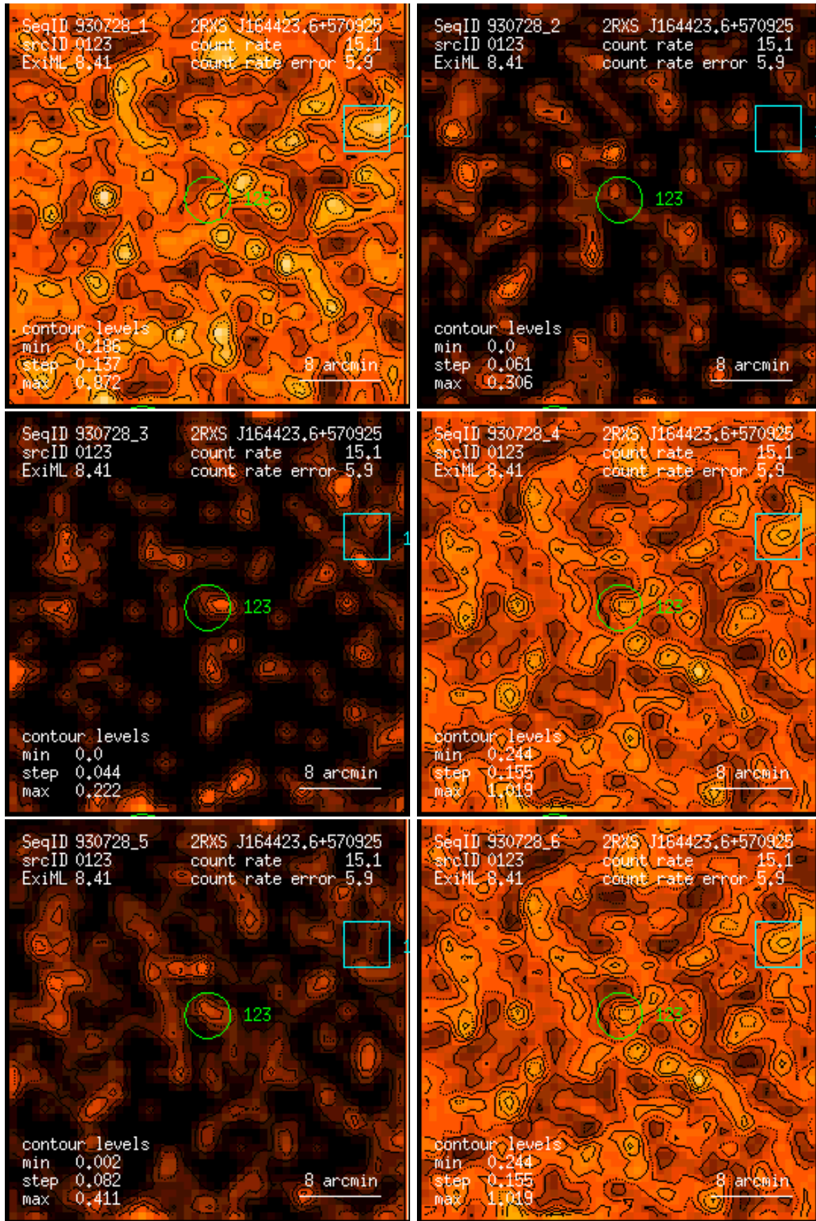
Figure 123: RASS 930728: detection 0123: band rate images, Gaussian filter: (1) PSPC channels 11 – 41, (2) 52 – 90, (3) 91 – 201, (4) 11 – 235, (5) 52 – 201, (6) 11 – 201. Broad band rates in counts/ks. Band rate contour levels in counts/ks/arcmin 2 .
