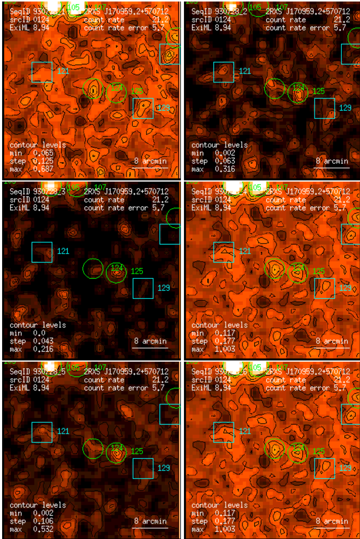
Figure 124: RASS 930728: detection 0124: band rate images, Gaussian filter: (1) PSPC channels 11 – 41, (2) 52 – 90, (3) 91 – 201, (4) 11 – 235, (5) 52 – 201, (6) 11 – 201. Broad band rates in counts/ks. Band rate contour levels in counts/ks/arcmin 2 .
