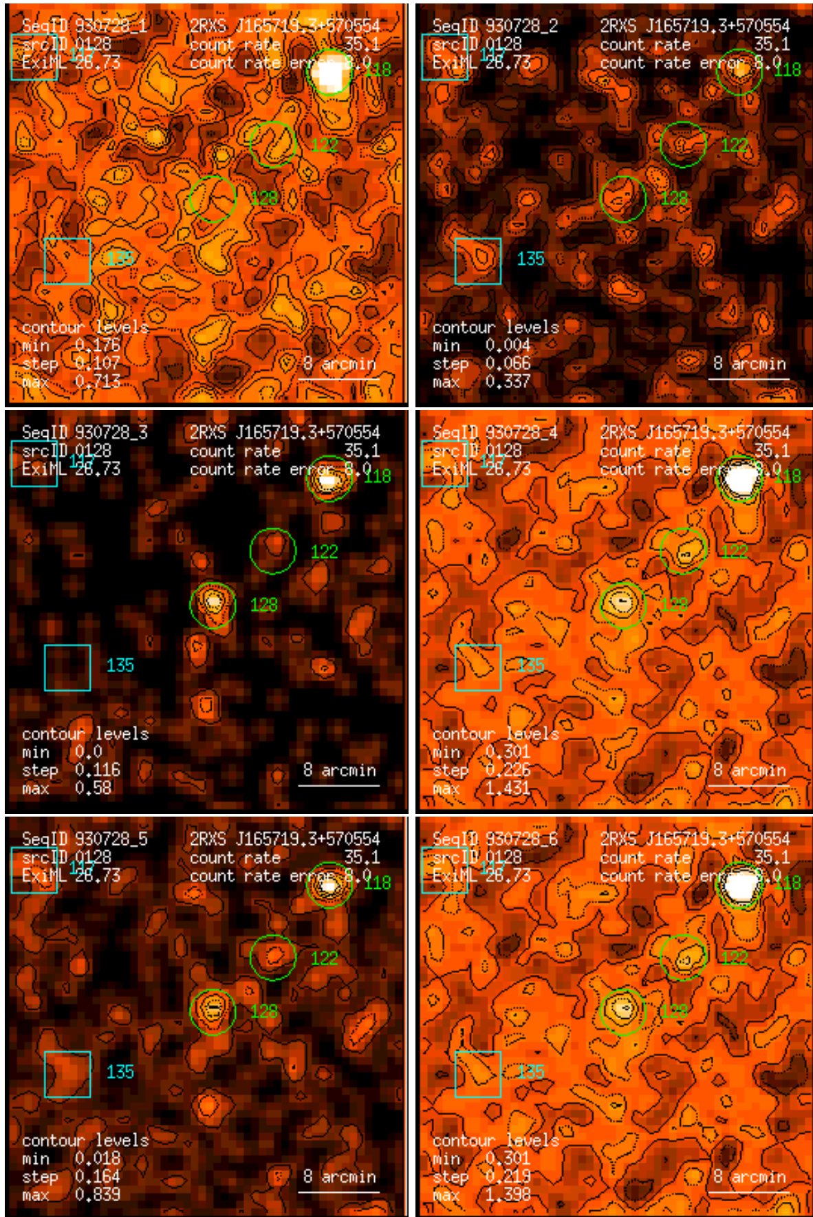
Figure 128: RASS 930728: detection 0128: band rate images, Gaussian filter: (1) PSPC channels 11 – 41, (2) 52 – 90, (3) 91 – 201, (4) 11 – 235, (5) 52 – 201, (6) 11 – 201. Broad band rates in counts/ks. Band rate contour levels in counts/ks/arcmin 2 .
