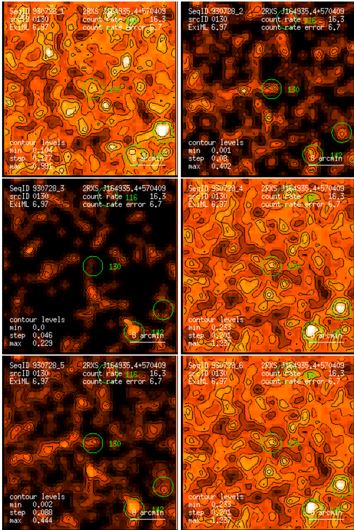
Figure 130: RASS 930728: detection 0130: band rate images, Gaussian filter: (1) PSPC channels 11 – 41, (2) 52 – 90, (3) 91 – 201, (4) 11 – 235, (5) 52 – 201, (6) 11 – 201. Broad band rates in counts/ks. Band rate contour levels in counts/ks/arcmin 2 .
