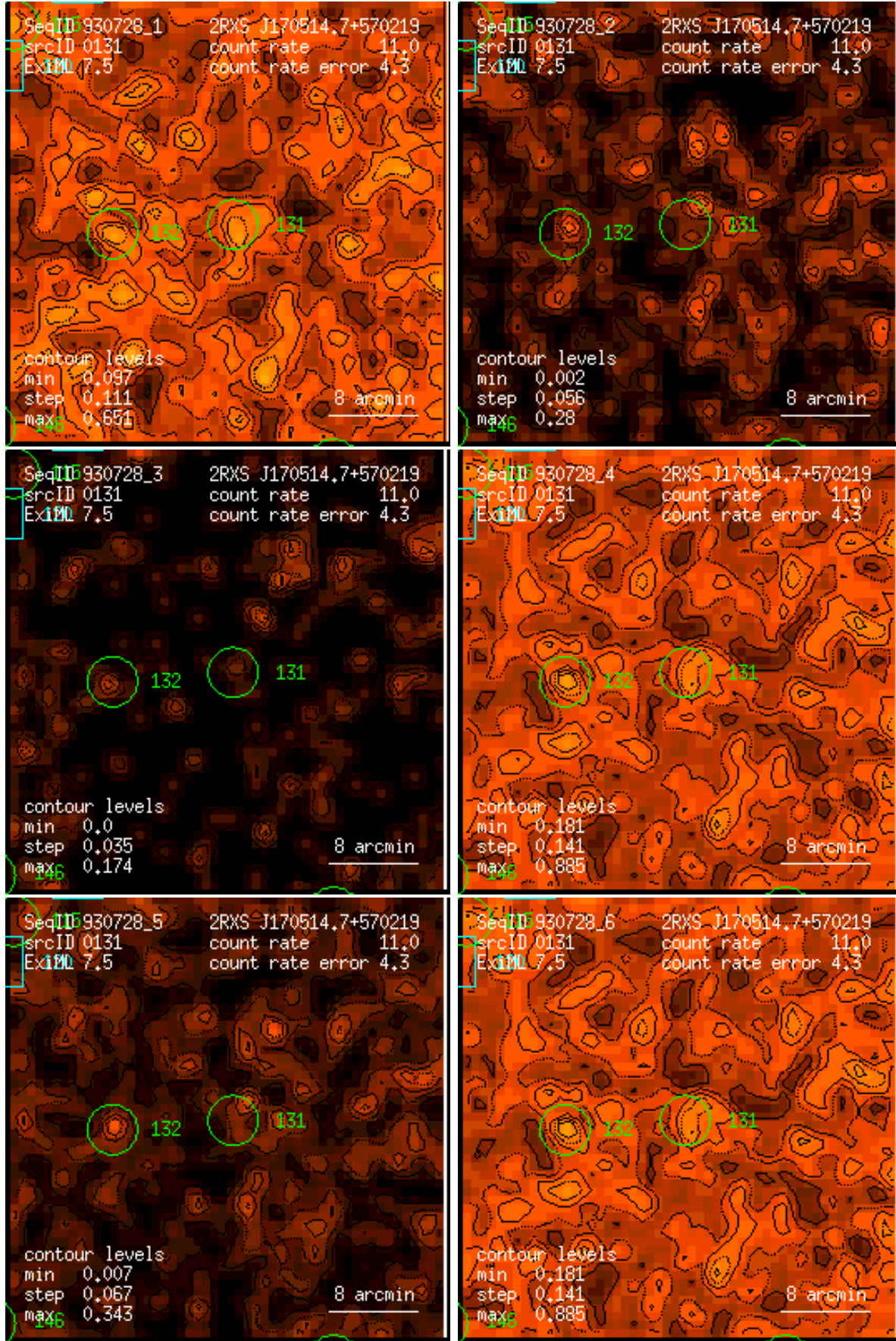
Figure 131: RASS 930728: detection 0131: band rate images, Gaussian filter: (1) PSPC channels 11 – 41, (2) 52 – 90, (3) 91 – 201, (4) 11 – 235, (5) 52 – 201, (6) 11 – 201. Broad band rates in counts/ks. Band rate contour levels in counts/ks/arcmin 2 .
