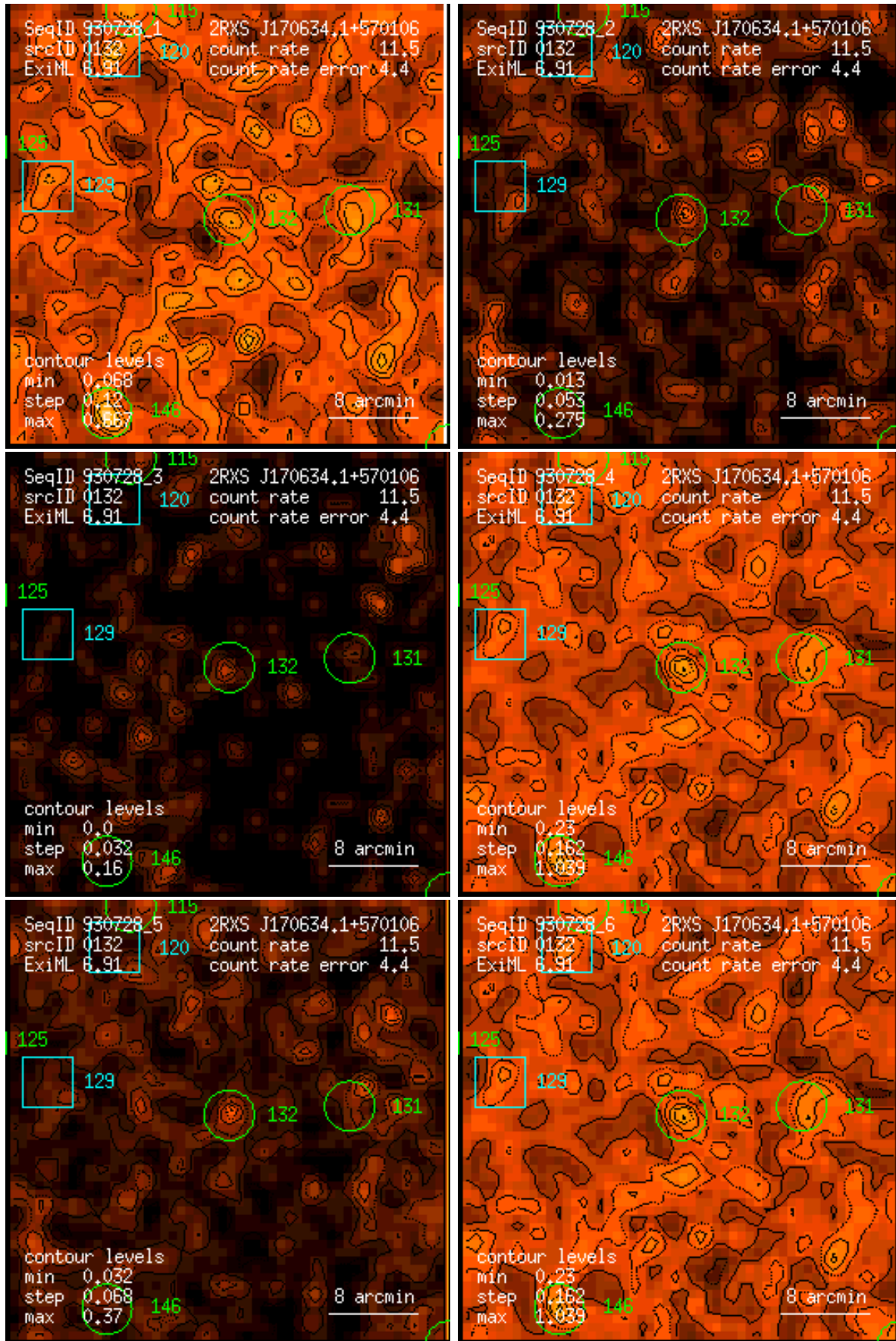
Figure 132: RASS 930728: detection 0132: band rate images, Gaussian filter: (1) PSPC channels 11 – 41, (2) 52 – 90, (3) 91 – 201, (4) 11 – 235, (5) 52 – 201, (6) 11 – 201. Broad band rates in counts/ks. Band rate contour levels in counts/ks/arcmin 2 .
